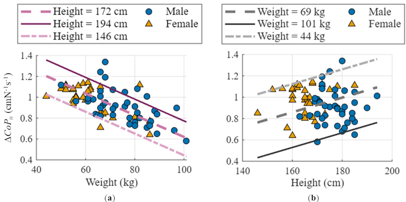
Fig. 5 Dependence of \Delta \text{CoP}_n on weight (a) and height (b) of the subjects. Purple lines represent linear regression lines calculated for different subject height values. Grey lines represent linear regression lines calculated for different subject weight values
