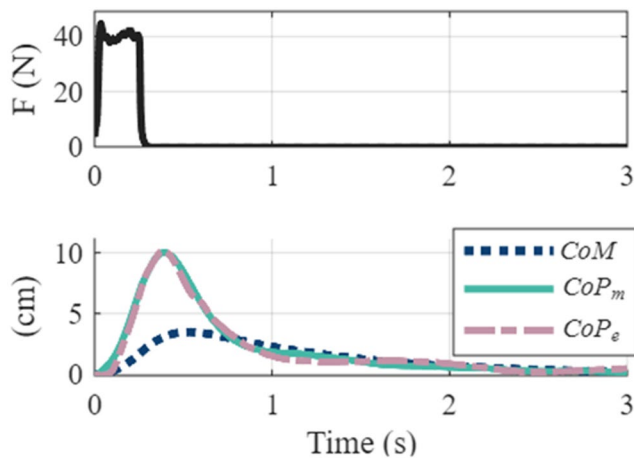
Fig. 6 Perturbation (top) and CoP fit (bottom) for a representative subject being modeled as SIP. CoP_e : average CoP response collected from the experimental recordings from the subject; CoP_m : simulated CoP response provided by the model; CoM : simulated CoM response
