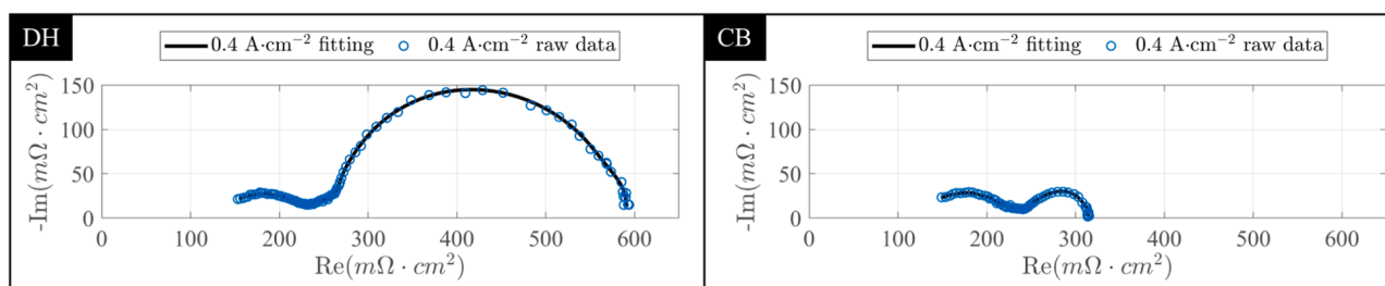
Fig. A.3. EIS fitting and raw data for DH environment and CB environment with full current density in the beginning of the durability test.
