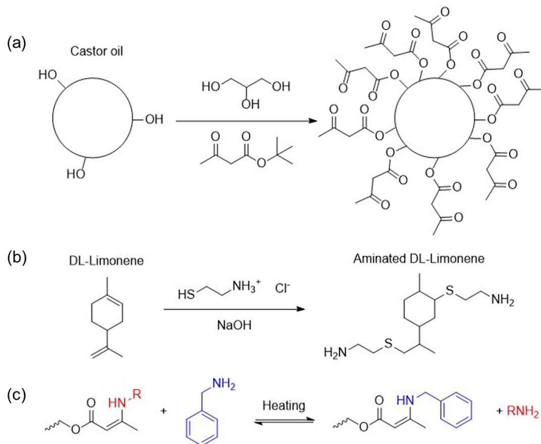
Fig. 18 Vitrimer derived from castor oil and DL-limonene: (a) synthetic route of the vinylidene urethane vitrimer, (b) synthesis of the aminated DL-limonene cross-linker, and (c) dissolution reaction in benzylamine at 120 °C. Adapted from ref. 114 with permission from Elsevier Ltd, Copyright © 2020.
