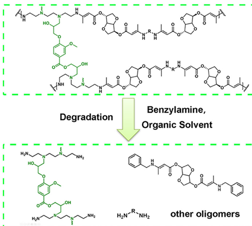
Fig. 8 Chemical degradation of bio-based vinylous urethane epoxy thermosets derived from isosorbide by immersion in ethanol for 24 h at room temperature with benzylamine. Reproduced from ref. 67 with permission from American Chemical Society, Copyright © 2023.
