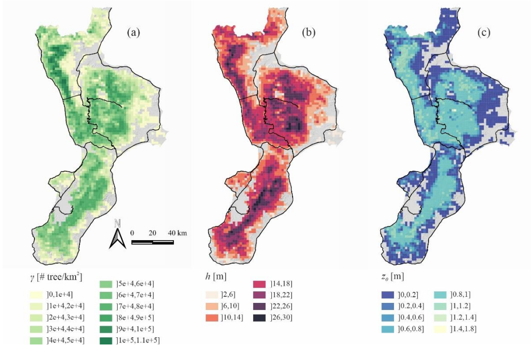
Figure 7. Mesoscale maps of tree canopy mean density \gamma (a), mean height h (b), and surface roughness z_0 (c) with common horizontal resolution L = 2.2 km according to [47], [48] and [29], respectively
