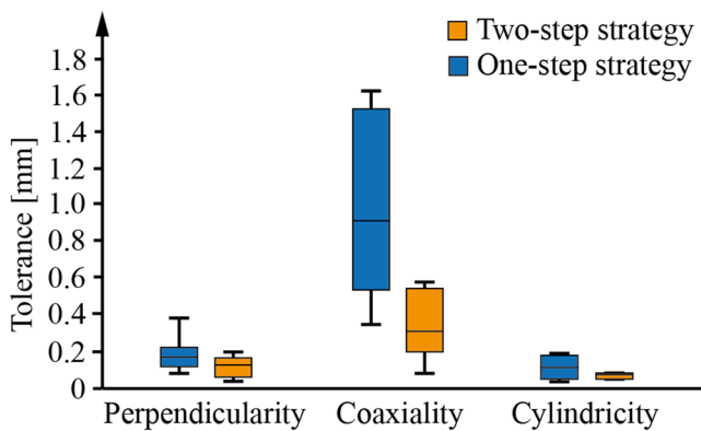
Fig. 12 Tolerance for Perpendicularity, coaxiality and cylindricity in the case of the two melting strategies
