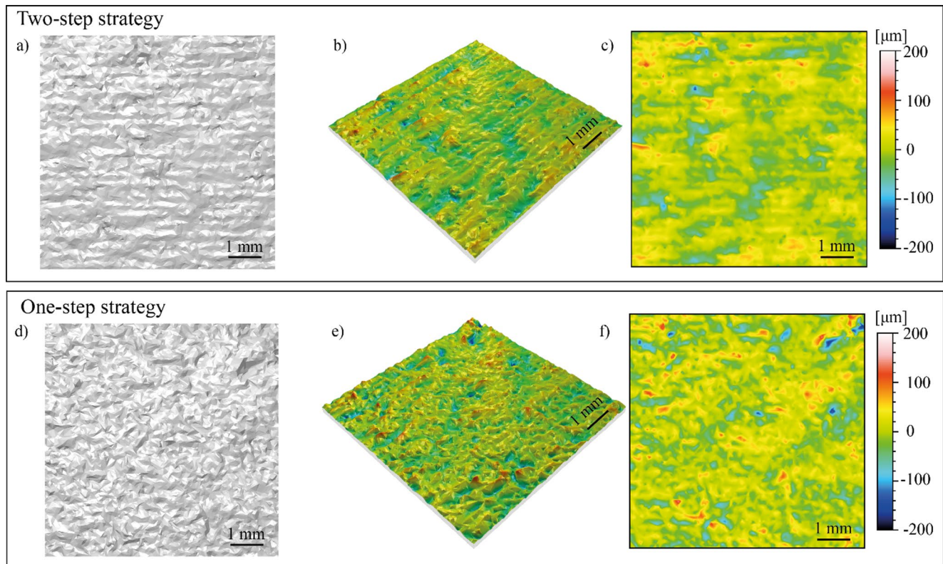
Fig. 7 Topography analysis of the horizontal surfaces. a–c refer to the surface produced with the two-step strategy, while d–f refer to surfaces produced with the one-step strategy. a, d Represent the unprocessed
