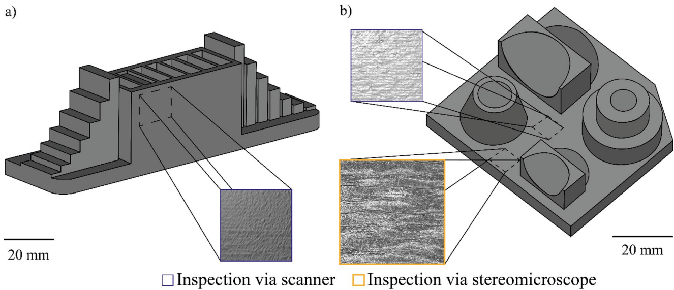
Fig. 3 Location of the areas for the surface topography characterisation. a Location for topography characterisation of vertical surfaces. b Location of the surface for characterisation of the horizontal surface and location of the melt track inspection location with the stereomicroscope
