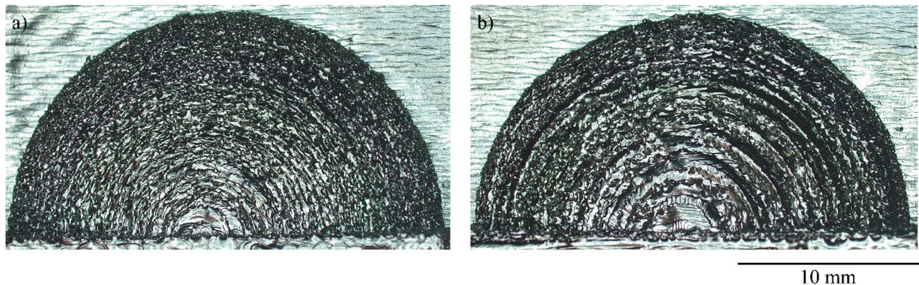
Fig. 5 Detailed image of the convex sphere SP1 of artefact 2 produced with two-step (a) and one-step (b) melting strategy
