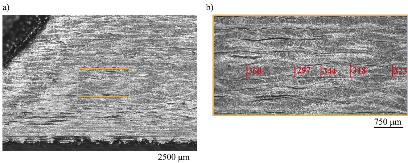
Fig. 8 a) Optical microscopy image of the top surface. b) Detail of the surface with measures of the width of the melt track in \mu\text{m}
