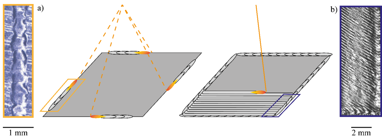
Fig. 1 Melting strategies in PBF-EB. a Contour melting and b hatch melting
