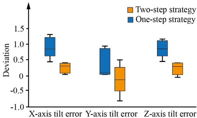
Fig. 13 Deviation of the angles with respect to the coordinate axes for the two-step and one-step melting strategy considered
