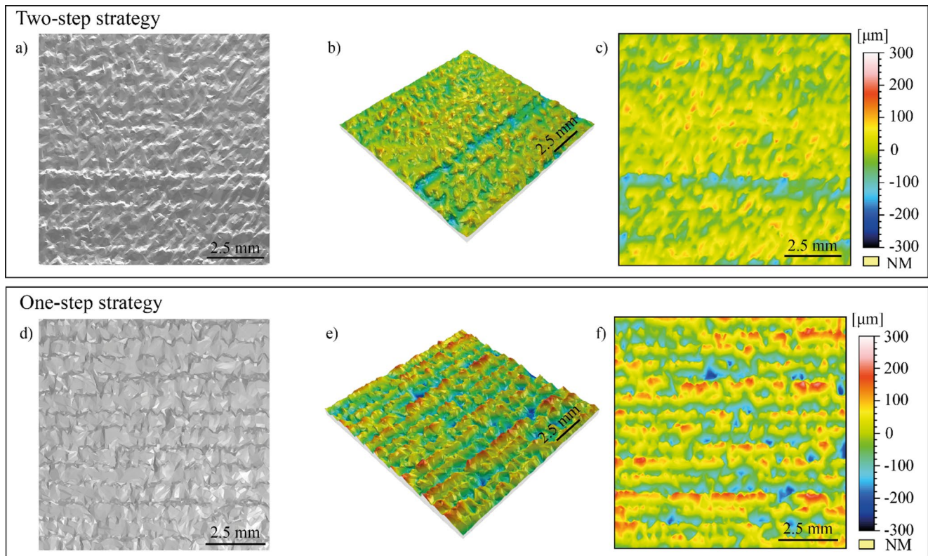
Fig. 6 Topography analysis of the vertical surfaces. a–c Refer to the surface produced with the two-step strategy, while d–f refer to the surface produced with the one-step strategy. a, d Represent the unpro-
