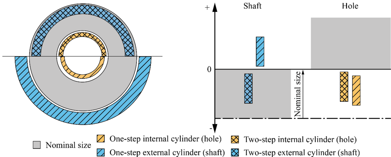
Fig. 10 Schematic representation of the tolerance interval and the relative position with respect to the nominal size. The dimensions are out of scale
