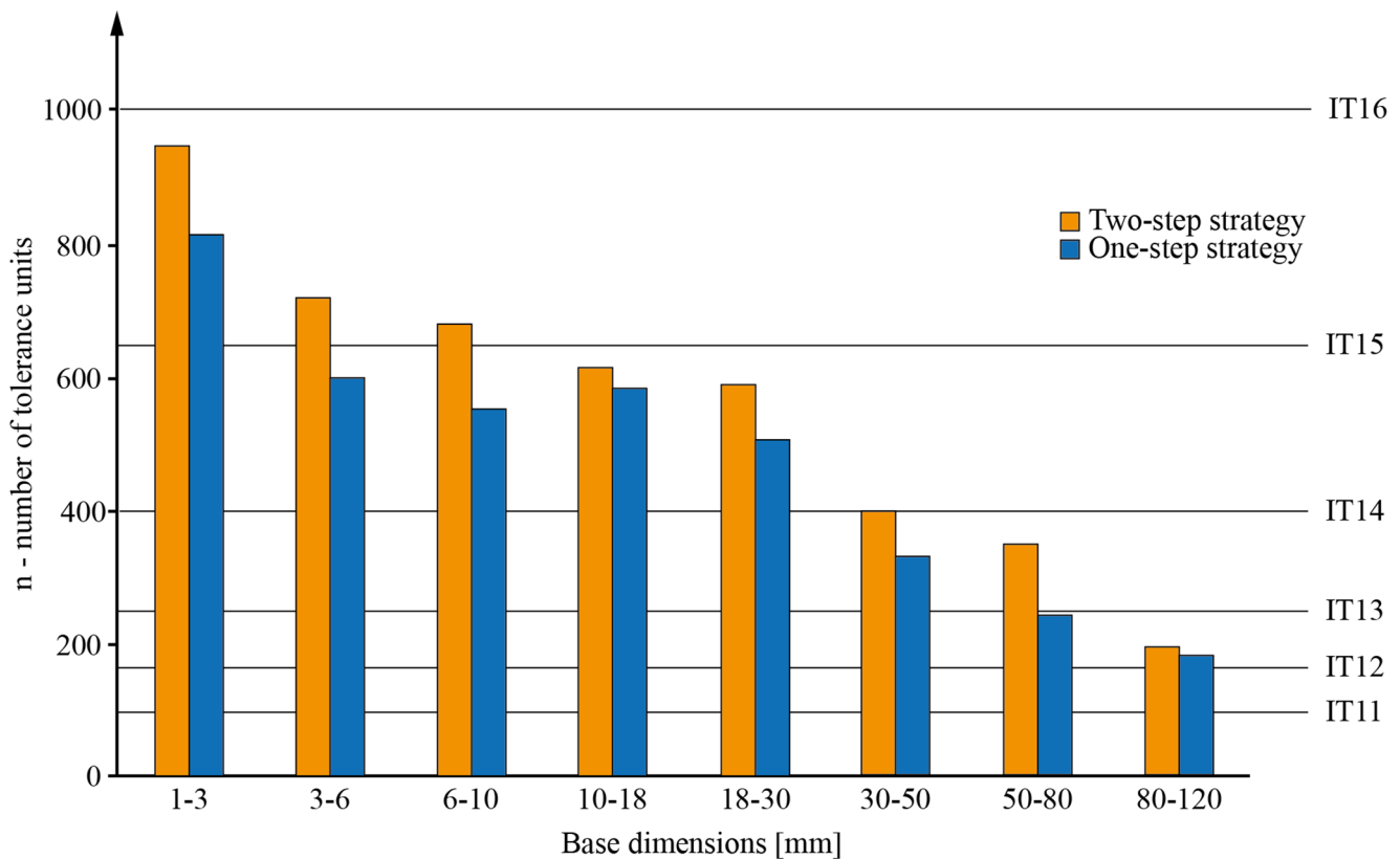
Fig. 9 Number of tolerance units for the artefacts produces using the Two-step strategy and the one-step strategy for the ISO base dimensions
