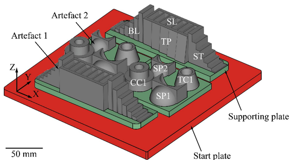
Fig. 2 Artefacts adopted to investigate the effect of the melting strategy and the relative position on the start plate. The quotes of the overall size are expressed in mm. The z-axis corresponds to the build direction
