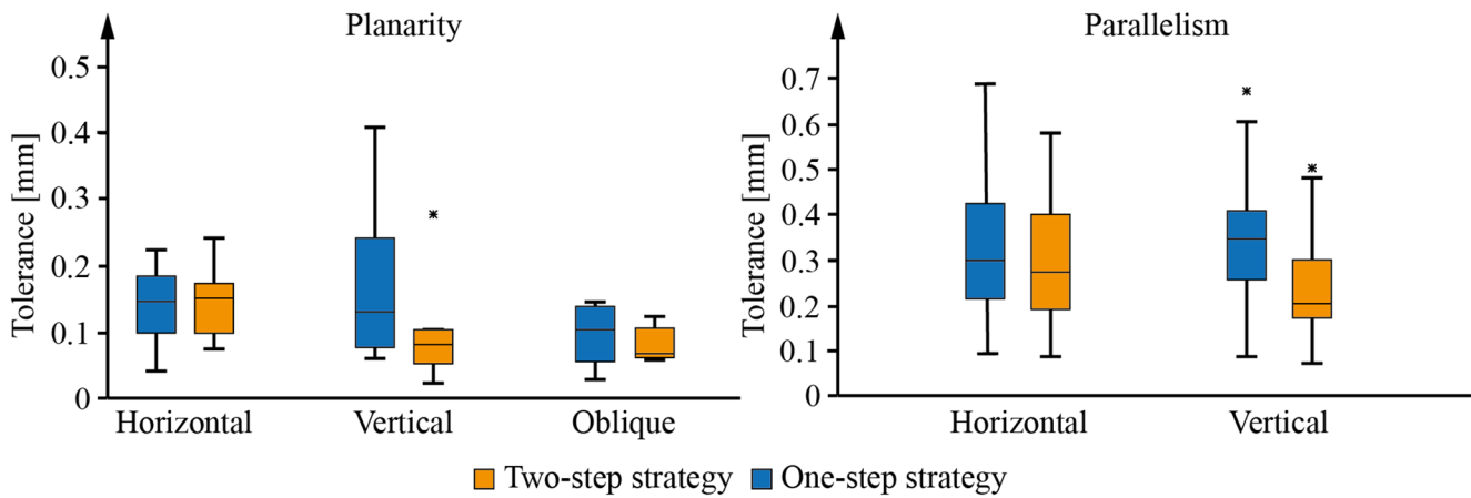
Fig. 11 Geometrical tolerances for planarity and parallelism
