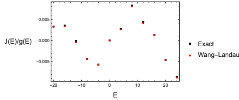
Figure 5: Equilibrium “microcanonical” current J(E)/g(E) (normalized by density of states for rendering reasons) as a function of energy E for U_2 = U_3 = 1 , \rho = 0.5 and N = 12 . Black squares: exact results; red circles: WL simulation results.
