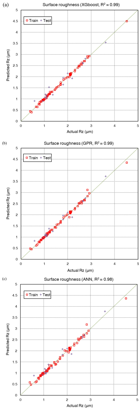
Fig. 6 Correlation between prediction and Actual Rz with ML model: a XGBoost; b GPR; c ANN
