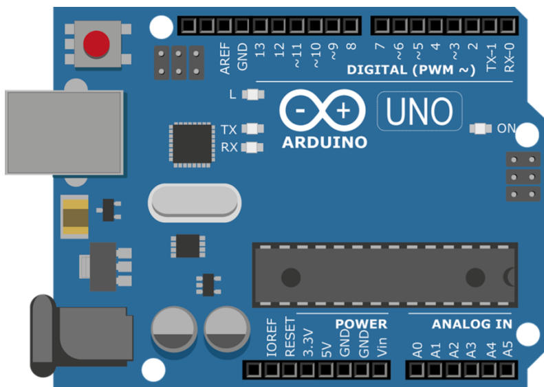
Fig. 17 - Arduino Uno Board (source: cleanpng.com ).
