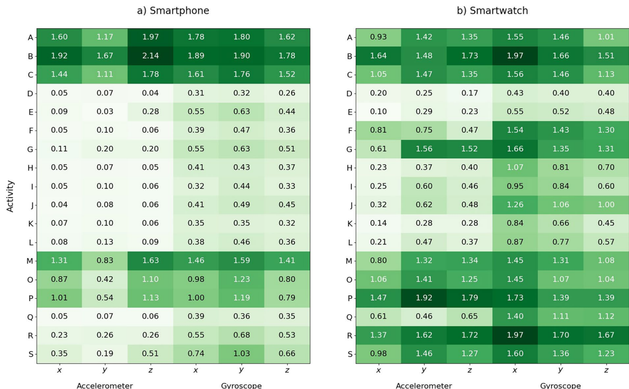
Fig. 3 Heatmaps of entropy measurements for smartphone (a) and smartwatch (b). The heatmaps illustrate the entropy values of the sensor signals. These values show that the accelerometer signals have lower entropy than the gyroscope signals in both devices.
