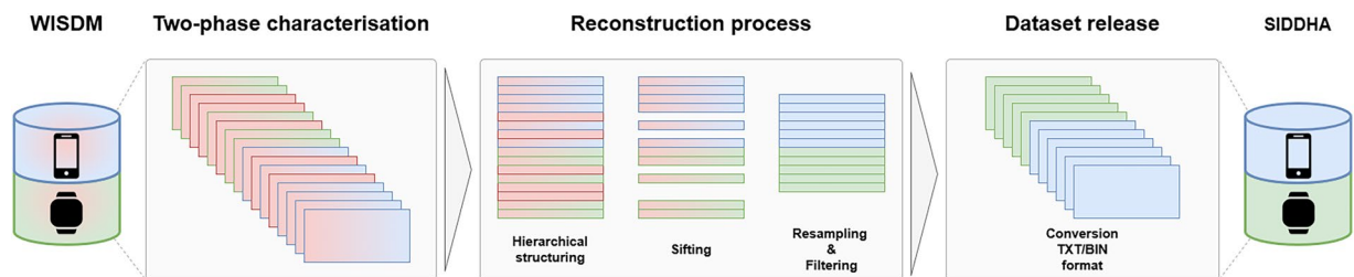
Fig. 1 Building blocks of the WISDM sample analysis and the reconstruction process for the SIDDHA production. We employ a two-step characterisation process in the initial phase to identify potential issues affecting individual instances or the entire dataset. In the second phase, we apply the reconstruction process through three steps: hierarchical structuring, which organises the data according to the source device, subject, activity class, and sensor type; sifting, which removes instances with incomplete sensor measurements; resampling and filtering, which reconstruct the signal, providing output instances with uniform sampling at 20 Hz. In the third phase, we convert the reconstructed instances that compose the SIDDHA dataset into binary and text formats.
