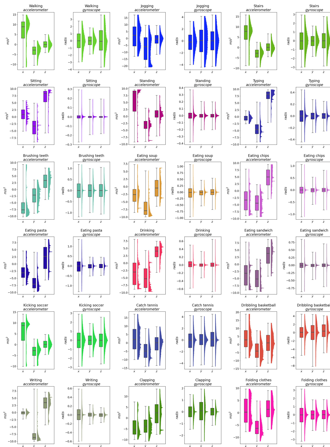
Fig. 6 The graphics illustrate the intensity distribution of the accelerometer and gyroscope measurements for each class recorded with a smartwatch. We obtained these values by analyzing the signals for each class across multiple subjects. Each class has a set of accelerometer and gyroscope graphics showing measurements along the x-, y-, and z-axes.
