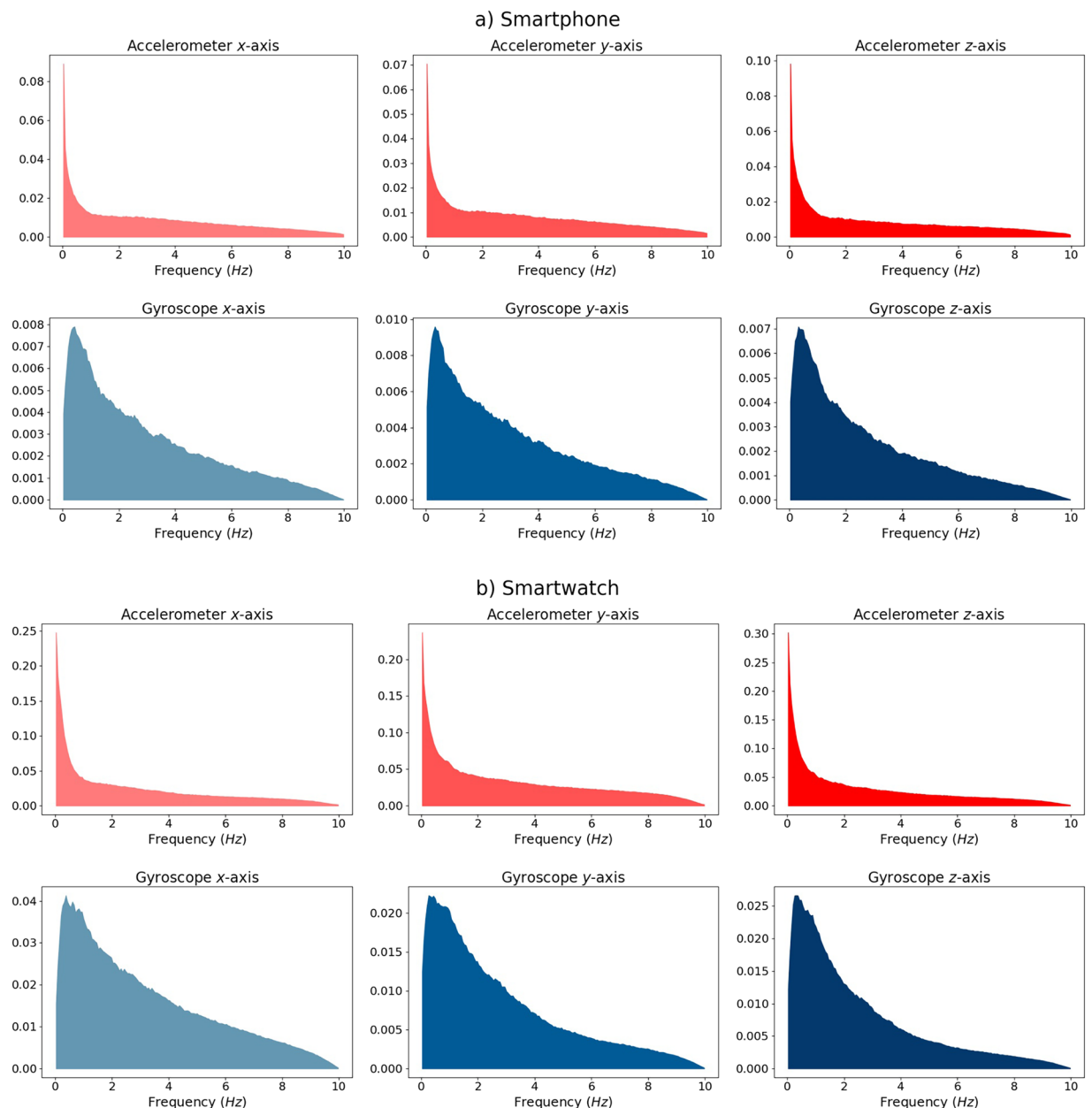
Fig. 4 The plots illustrate a comparison of the frequency spectrum for smartphone (a) and smartwatch (b). The spectra are obtained through the median of the Fourier transform on all the available classes of users that compose the dataset. The accelerometer and gyroscope are reported at the top and bottom of Figures (a) and (b), respectively. In this case, a wider distribution is observed for the spectrum belonging to the gyroscope sensor.
