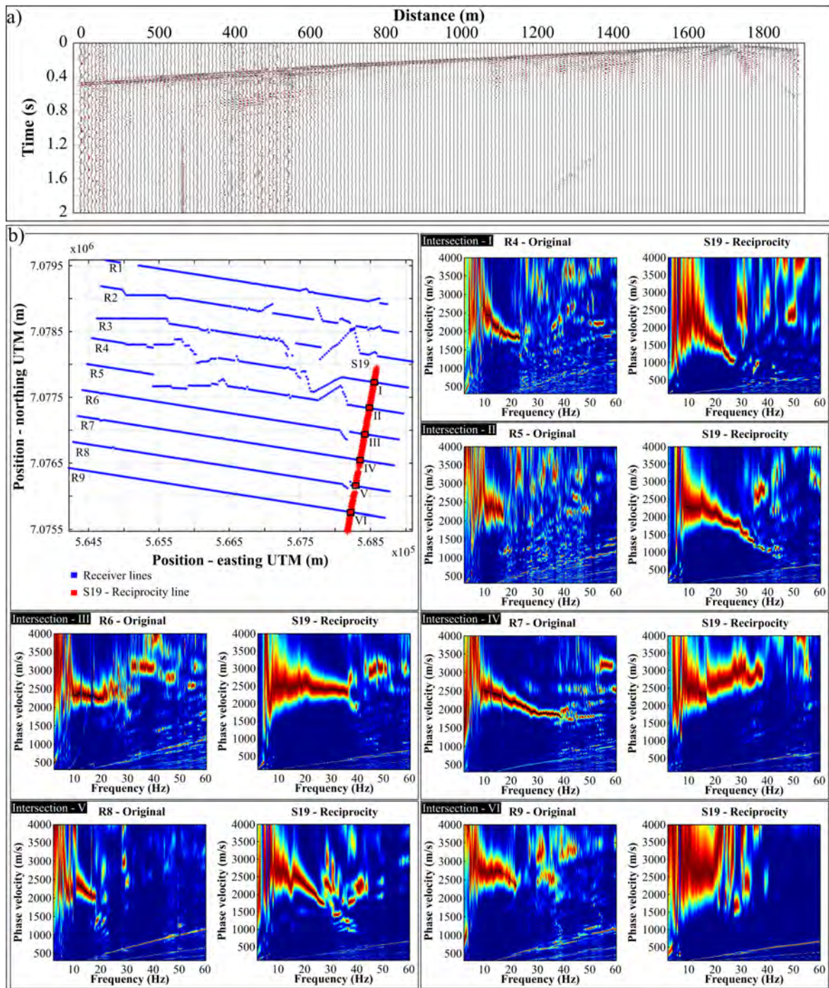
Figure 6. (a) Example of a common receiver gather obtained along source line S19. (b) Receiver and source line f-v spectra obtained at intersection locations I–VI.
