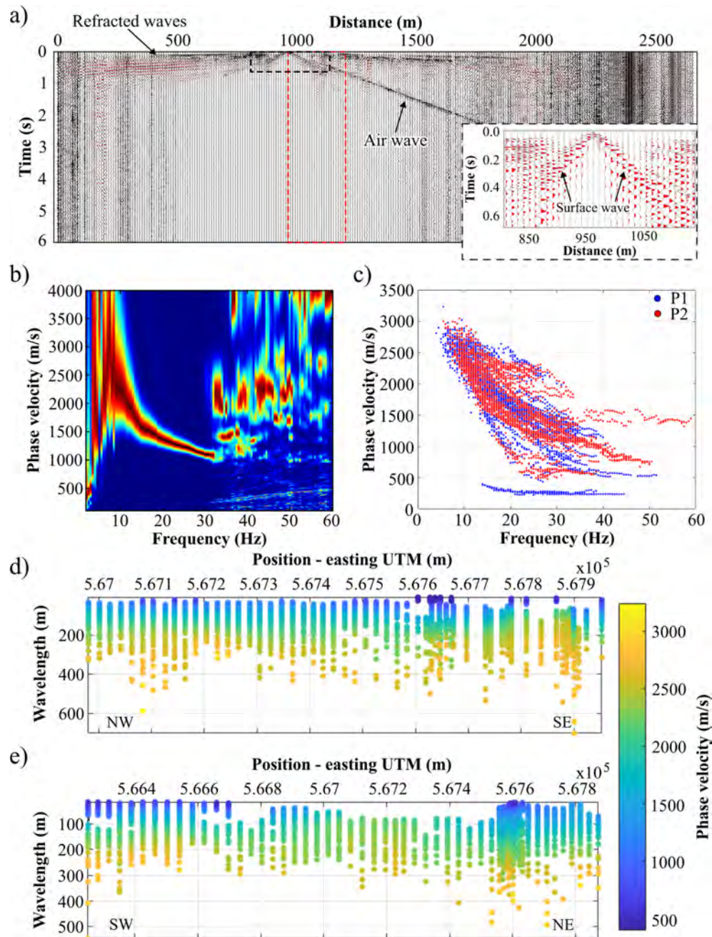
Figure 4. (a) Shot gather from the seismic profile P2, showing the window position (red dashed rectangle) that is later transformed into the frequency-phase velocity domain. A zoomed in window showing the surface wave trend visible in the record is shown, and its location is indicated using a dashed black rectangle. (b) Frequency-phase velocity spectrum from P2 obtained after transforming the highlighted data in (a), where the black dots depict the picked dispersion curve. (c) Picked surface wave dispersion curves for profiles P1 (dark blue) and P2 (red), plotted as a function of frequency and phase-velocity. In (d) and (e), surface wave dispersion curves for profiles P1 and P2 are plotted as a function of wavelength depth and spatial location.
