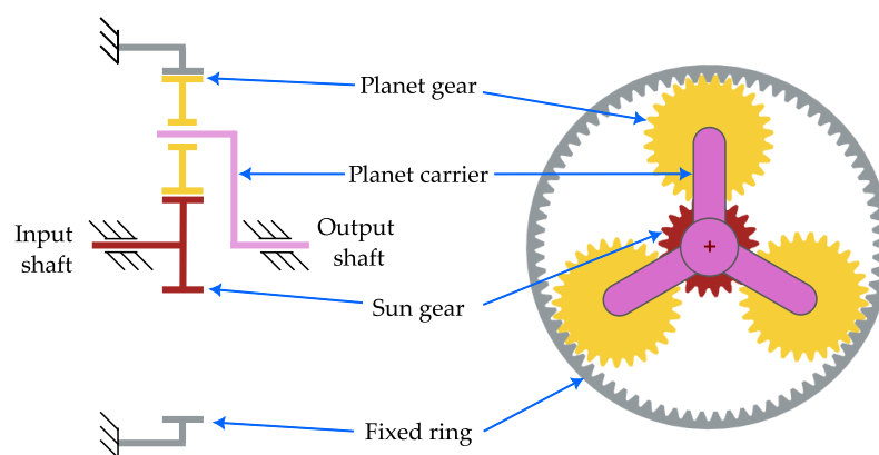
Figure 5. Planetary drive architecture.
