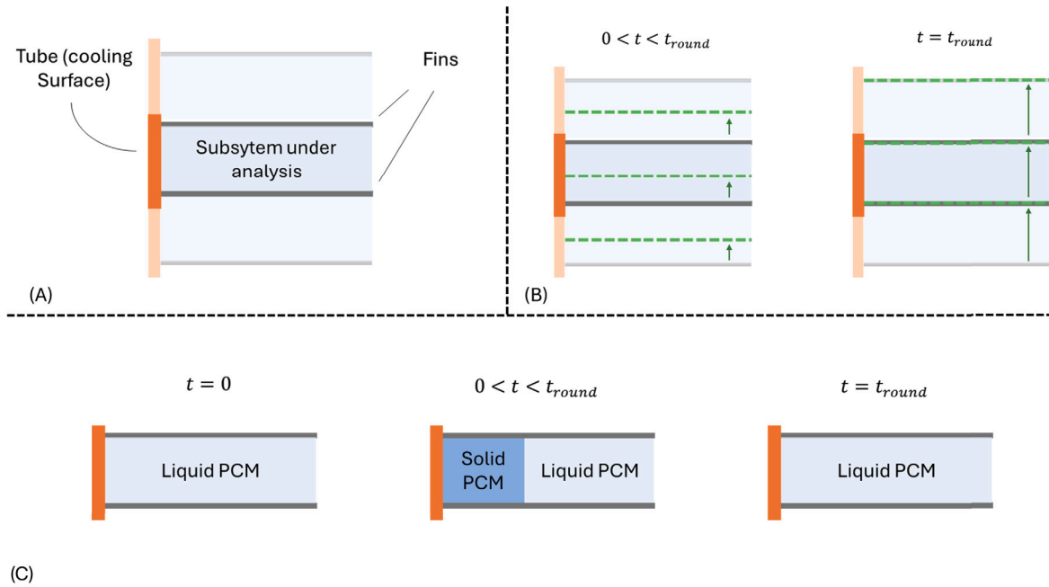
Fig. 4. Schematic of the simplified numerical analysis adopted for the dynamic case. (A) Subsystem under analysis, (B) vertical movement of the fins in the analyzed time frame 0 < t < t_{round} , (C) and schematic behavior of the solidification process in the considered simplified model.
