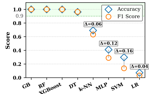
Fig. 2. Accuracy and F-1 score of various models
