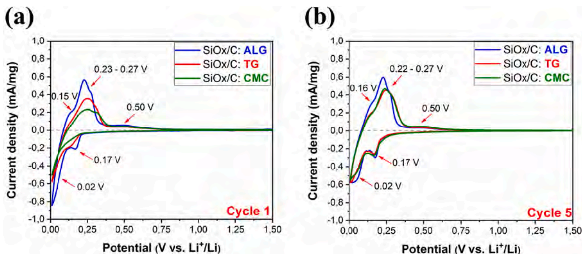
Fig. 3. Cyclic voltammetry at a scan rate of 0.1 mV/s of electrodes with all components (binder, active material, and conductive material) at cycle 1 (a) and cycle 5 (b).
