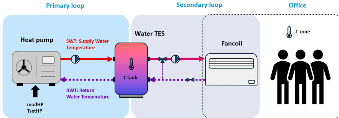
Fig. 1. Schematic representation of the considered heating system.
