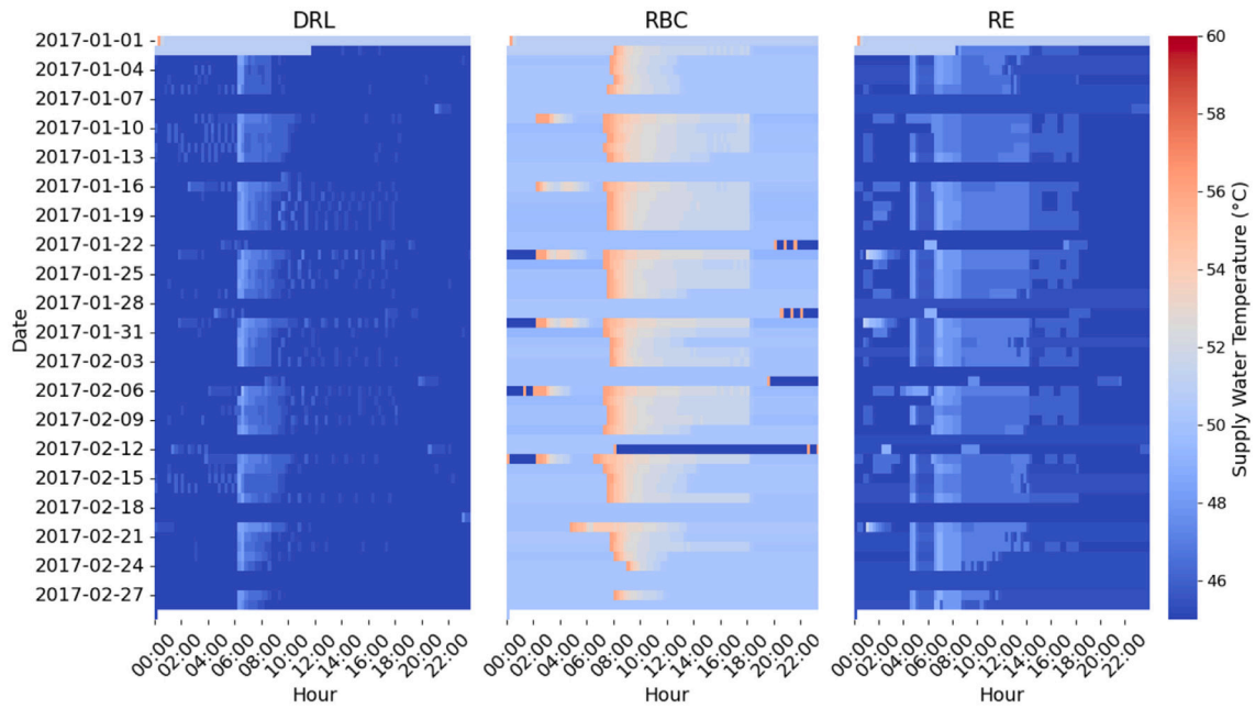
Fig. 13. Comparison of supply water temperature setpoints for the RBC, DRL, and RE controllers over the testing episode in the reference scenario.
