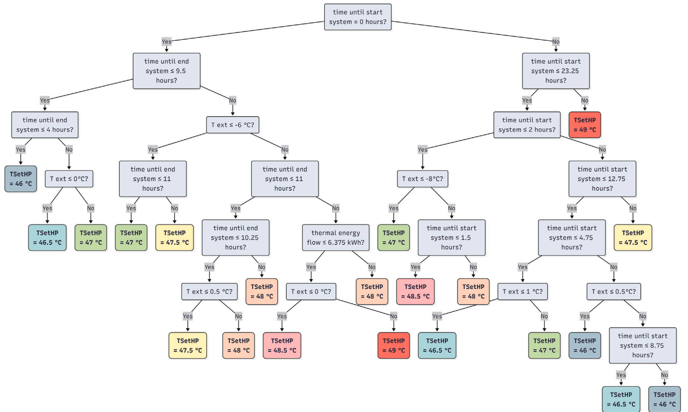
Fig. 9. Regression tree for the estimation of the TSetHP action.
