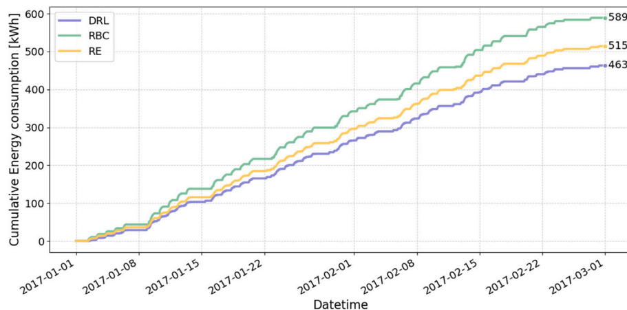
Fig. 11. Cumulative electrical energy consumption over the testing episode achieved by the RBC, DRL and RE controllers in the reference scenario.
