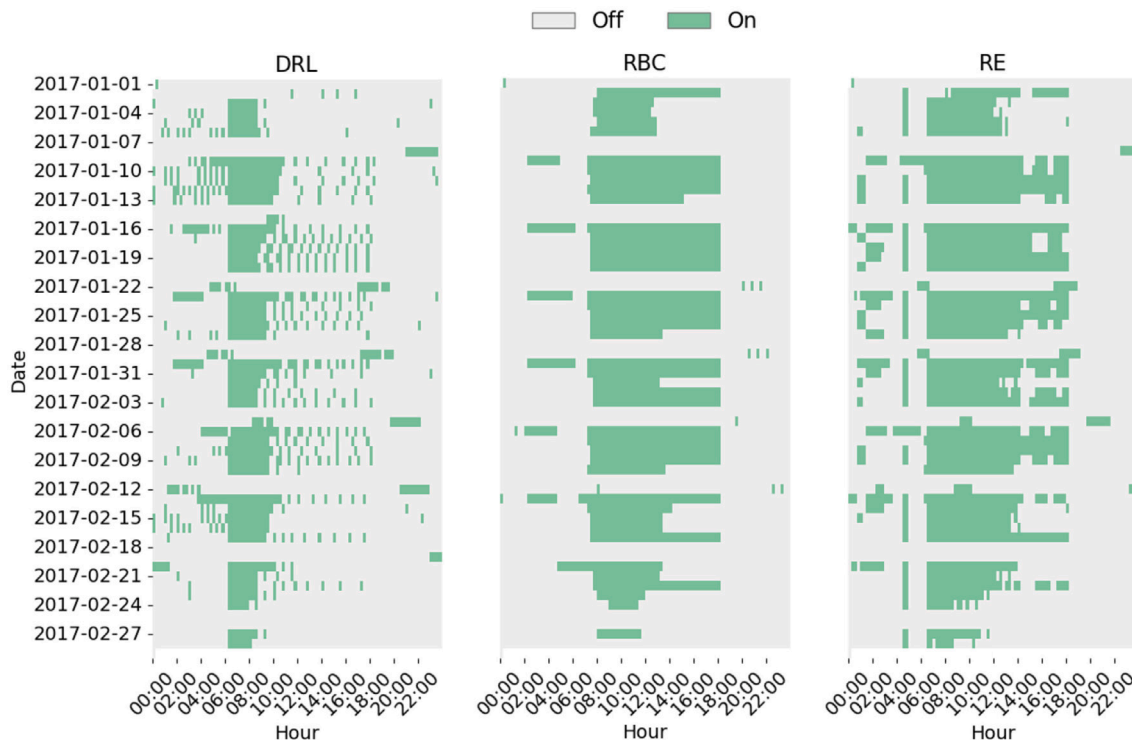
Fig. 12. Comparison of modHP actions for the RBC, DRL, and RE controllers over the testing episode in the reference scenario.
