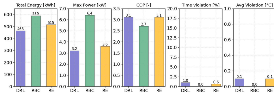
Fig. 10. Comparison between RBC, DRL and RE controller according to different KPIs in the reference scenario.
