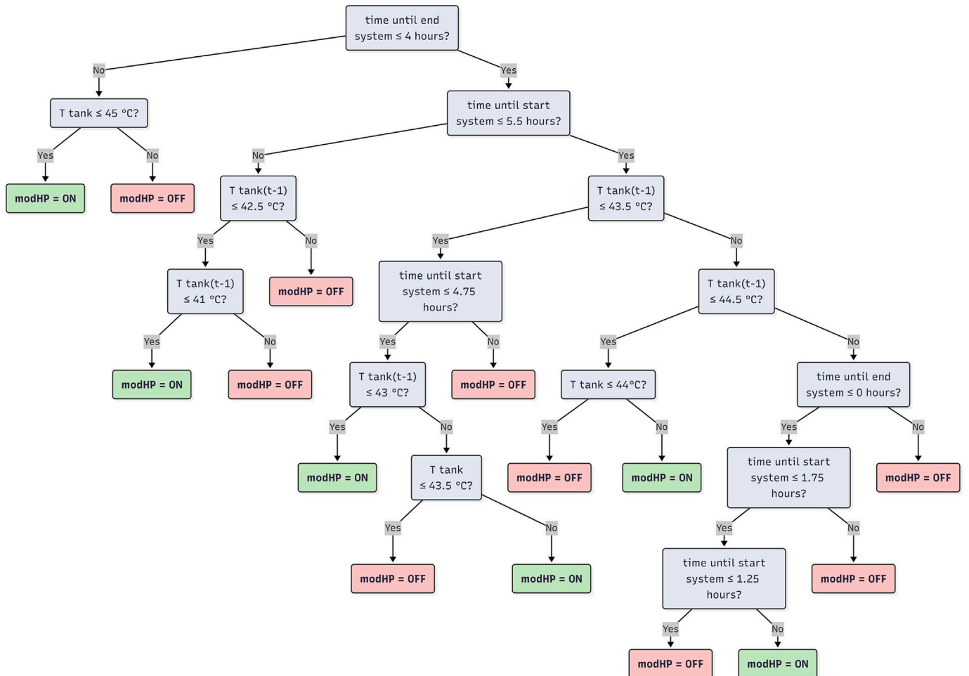
Fig. 8. Classification tree for the estimation of modHP action.
