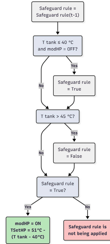
Fig. 5. Logic of the safeguard control rule.
