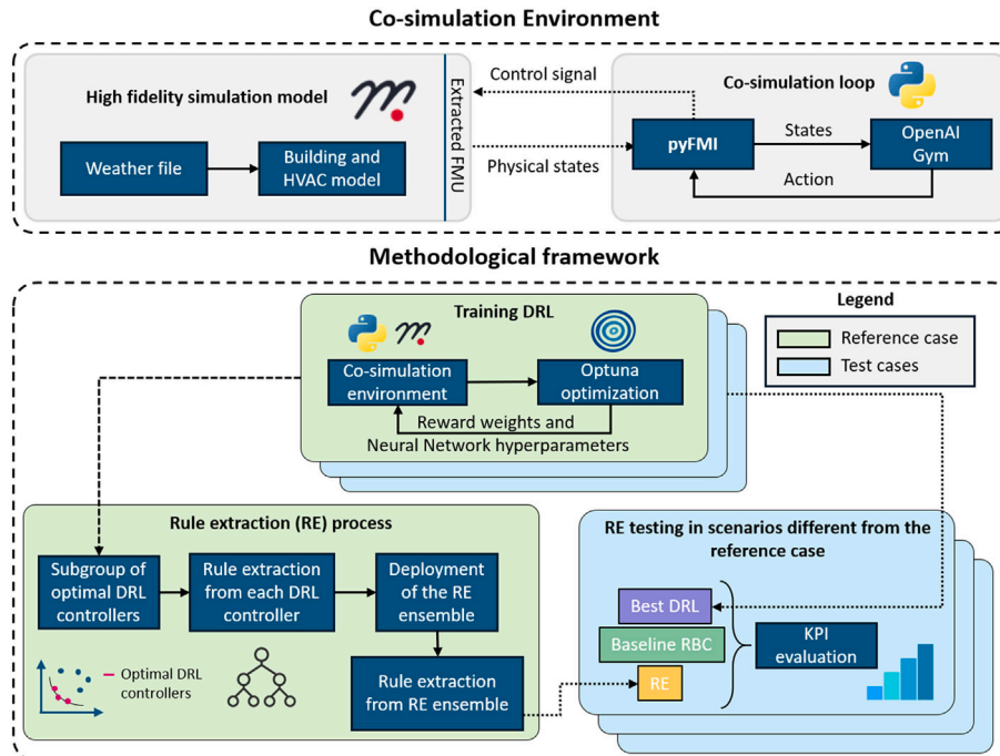
Fig. 3. Methodological framework.
