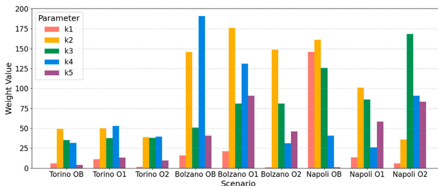
Fig. 7. Optimized reward weights for the best-performing DRL controller in each scenario.
