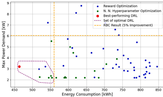
Fig. 6. Performance of different DRL agents in terms of energy consumption (x-axis) and max power demand (y-axis) during the deployment episode.
