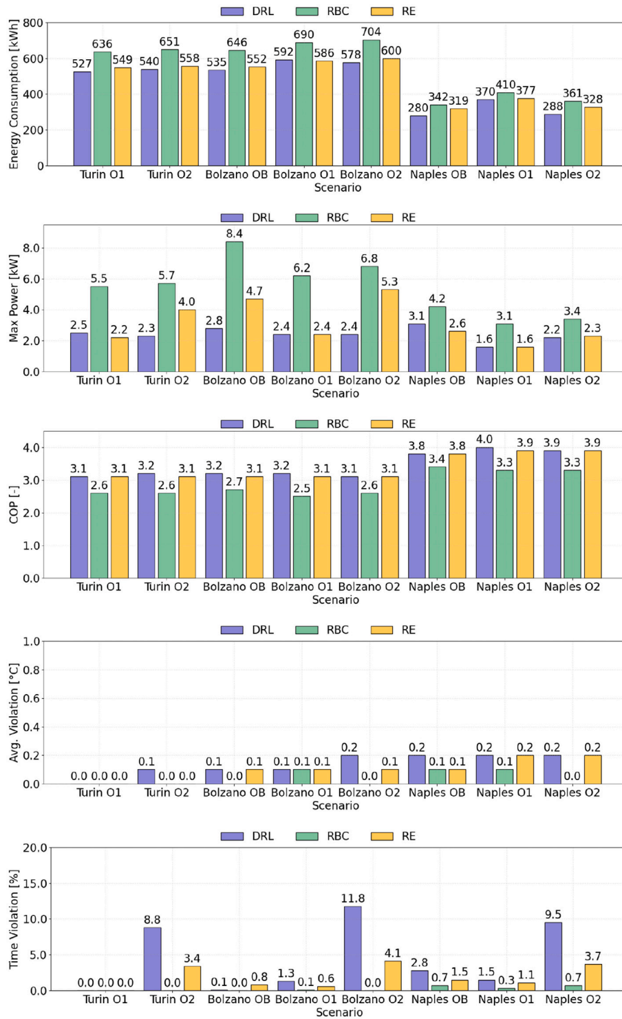
Fig. 14. Comparison between RBC, DRL and RE controller according to different KPIs in the transfer scenario.
