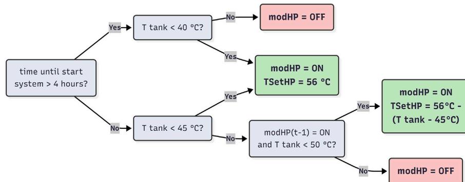
Fig. 2. RBC control logic.
