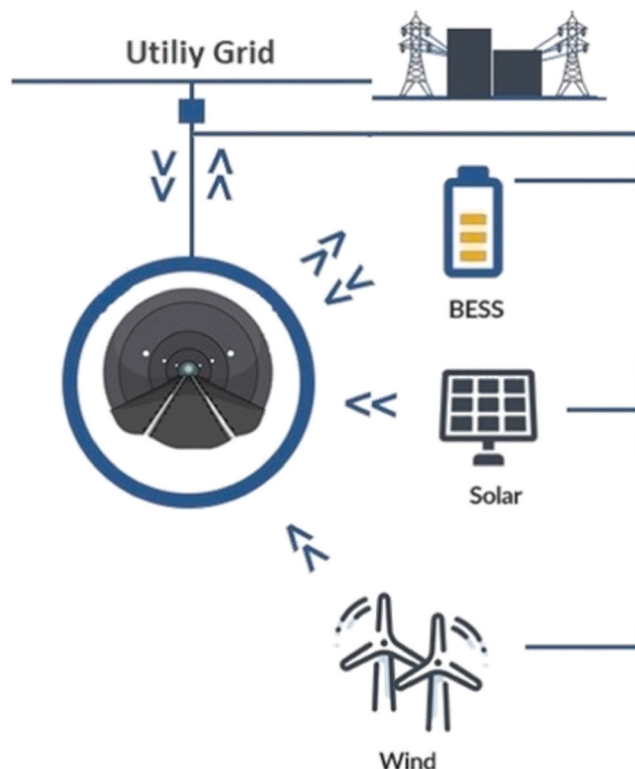
Fig. 1. Simplified scheme of the proposed MG for road tunnels.
