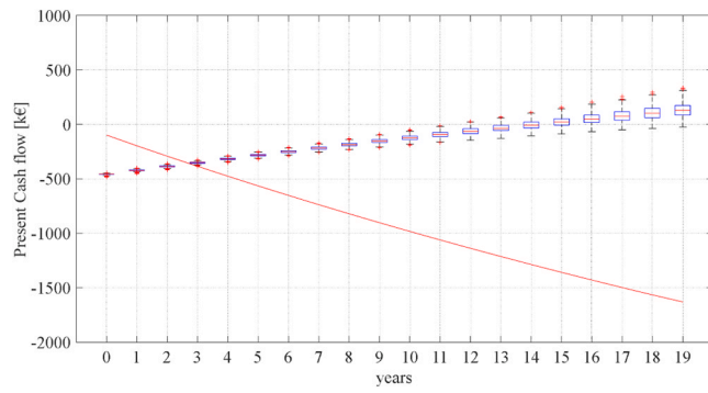
Fig. 12. Case study 2: boxplot of annual cash flow of the best solution with MG that includes renewable generators and storage systems and cash flow (red line) of road tunnel without DERs.
