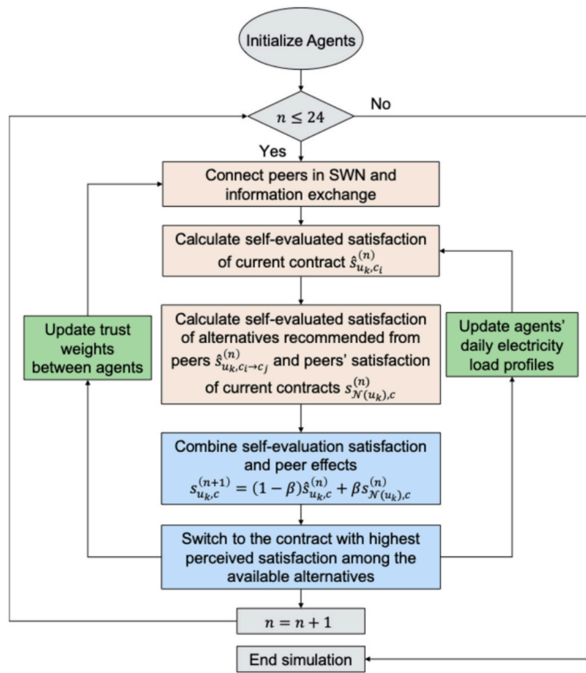
Fig. 3. Agent-based simulation of contract switching process.
