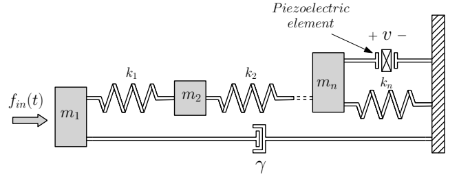
Fig. 1. Schematic representation of a networked multi-DOF resonator for energy harvesting applications.
