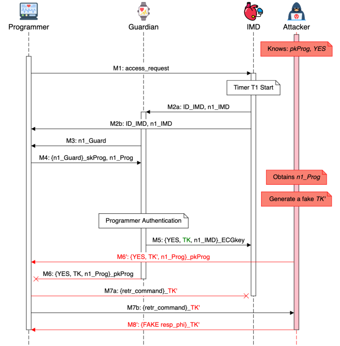
Figure 4. Attack Trace: an adversary exploits the flawed authentication to install a forged session key and deliver falsified PHI to the Programmer
