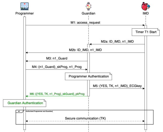
Figure 5. Fixed Regular Mode: Sequence Diagram
