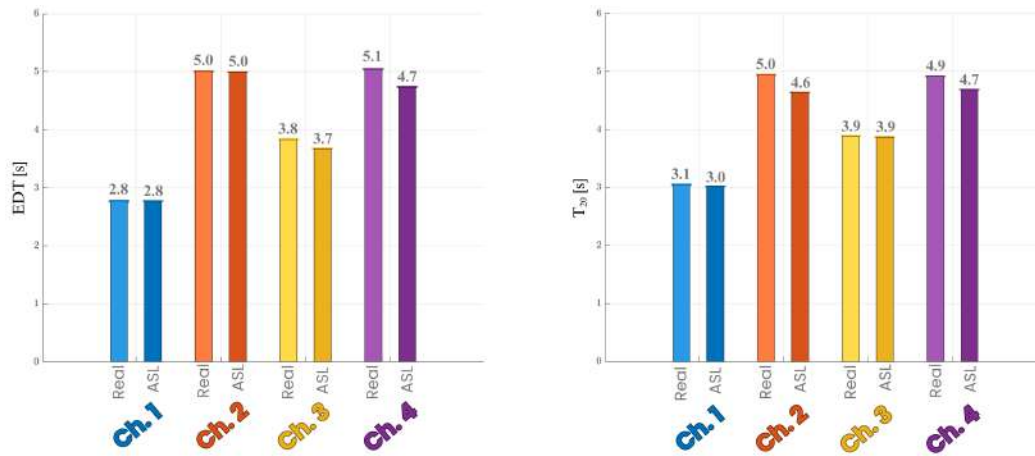
Figure 5: Comparison between EDT(left) and T_{20} (right) measured in the reference position in the four churches (Real) and in the Audio Space Lab (ASL)
