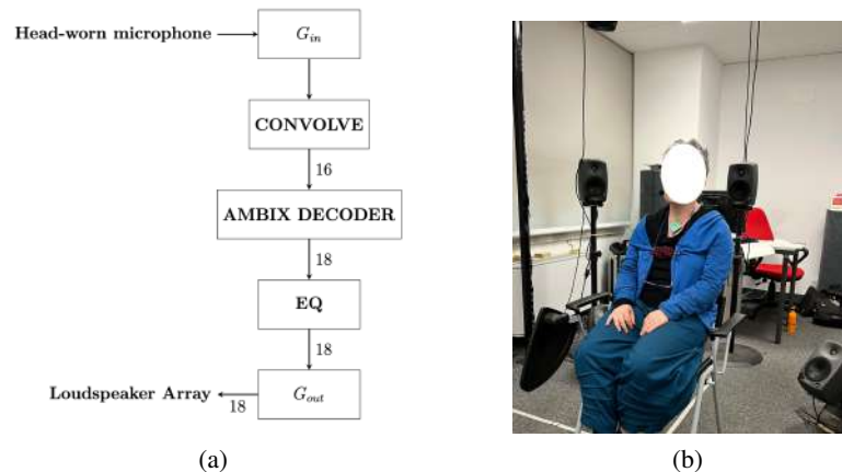
Figure 7: (7a): Block Diagram of the Real-Time Auralization System; (7b): Example of user singing in the ASL with the head-worn microphone
