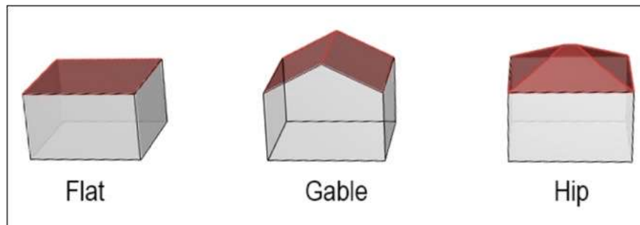
Fig. 3. Flat, gable, and hip roof types classified using GIS workflow.
