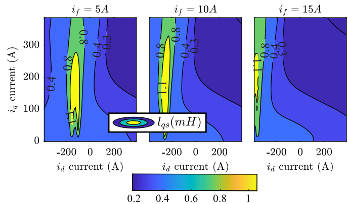
Fig. 16: Current-to-inductance l_{qs} map for the EESM under consideration.
