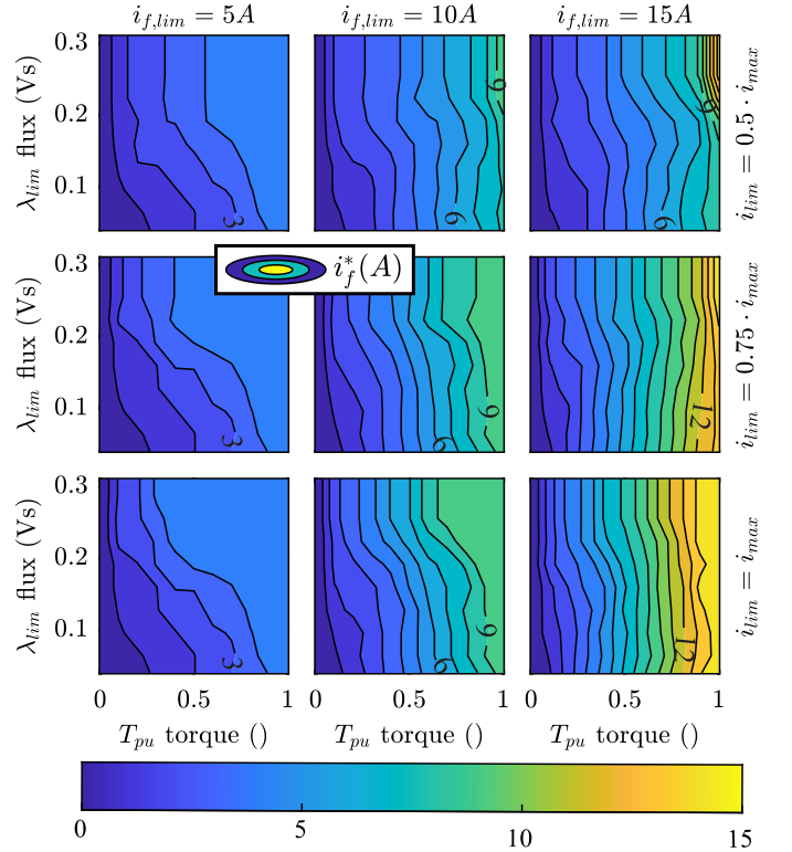
Fig. 14: Rotor current reference i_f^* maps (LUT6) for different stator and rotor current limits for the EESM under consideration.
