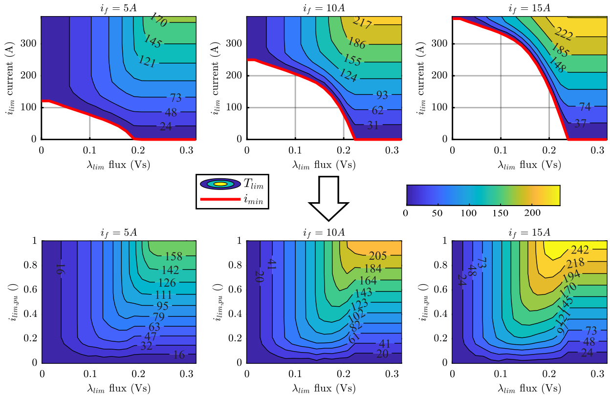
Fig. 10: Graphical view of the torque limit map (LUT3) transformation process for the EESM under consideration.
