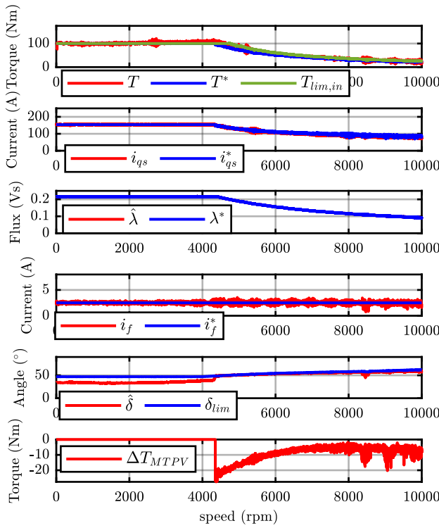
Fig. 24: MTPV limitation: experimental results.
