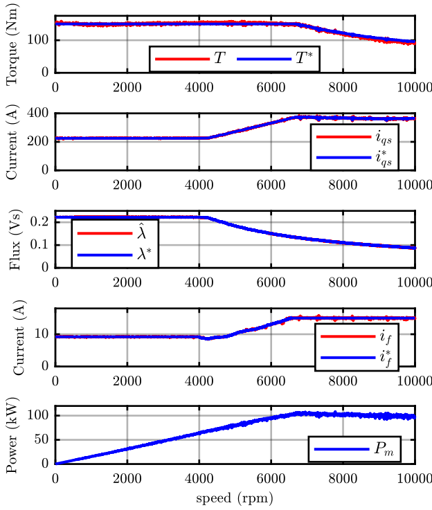
Fig. 19: MTPS profile at motoring: experimental results.
