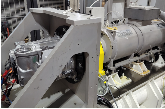
Fig. 18: View of the test rig: EESM under test (left), driving machine (right).
