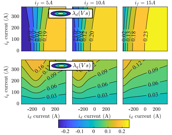
Fig. 5: Current-to-flux maps for the EESM under consideration.
