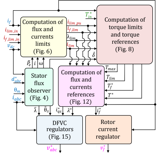
Fig. 3: Schematic view of the proposed torque controller.
