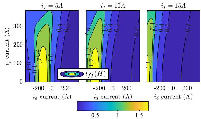
Fig. 17: Current-to-inductance l_{ff} map for the EESM under consideration.
