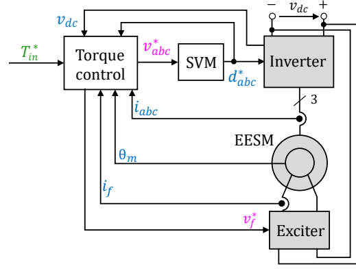
Fig. 1: Schematic view of EESM drive topology.
