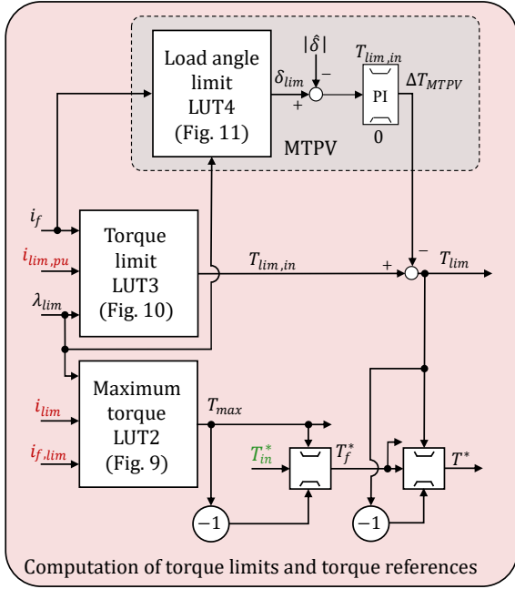
Fig. 8: Schematic view of the computation of torque limits and torque references.
