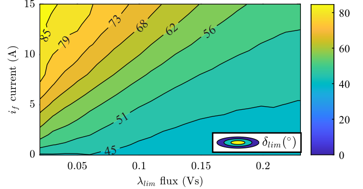
Fig. 11: Load angle limit map (LUT4) for the EESM under consideration.
