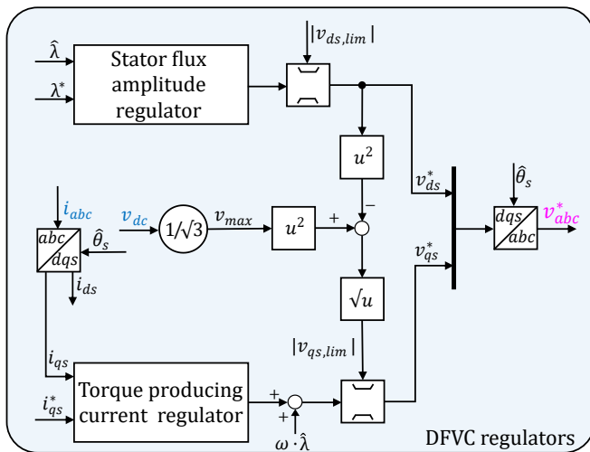
Fig. 15: Schematic view of the DFVC: closed-loop control of the stator flux amplitude and torque-producing current.
