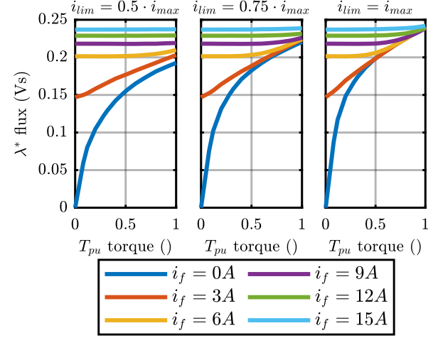
Fig. 13: Flux amplitude reference \lambda^* (LUT5) for different stator current limits and rotor current for the EESM under consideration.
