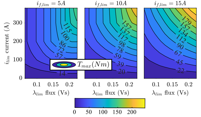
Fig. 9: Maximum torque map (LUT2) for the EESM under consideration.
