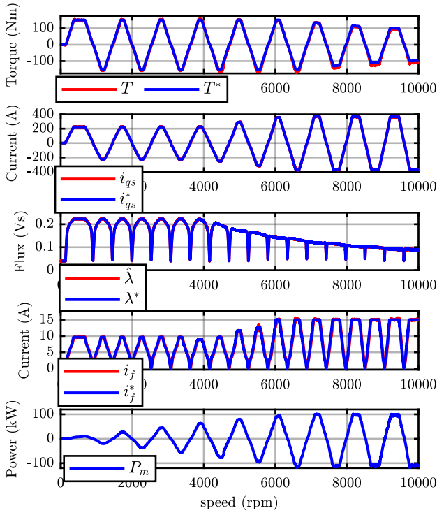
Fig. 21: Fast torque reversals along the MTPS profile: experimental results.
