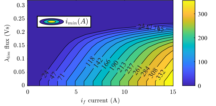
Fig. 7: Minimum stator current amplitude map (LUT1) for the EESM under consideration.
