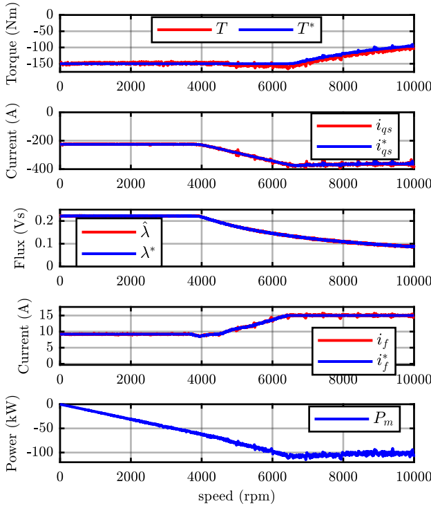
Fig. 20: MTPS profile at braking: experimental results.
