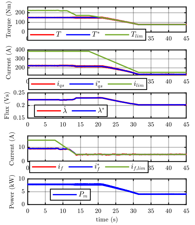
Fig. 23: Online variation of the current limits: experimental results.
