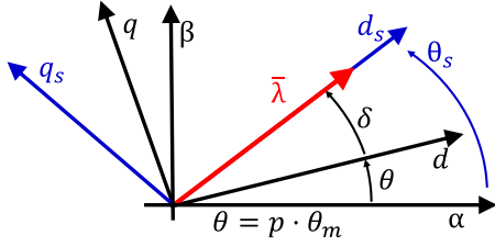
Fig. 2: Schematic view of the stationary- \alpha\beta , rotor- dq , and stator- dqs frames for a generic ac motor.
