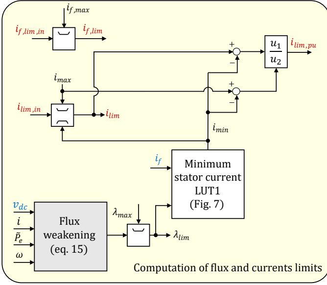
Fig. 6: Schematic view of the computation of flux and current limits.
