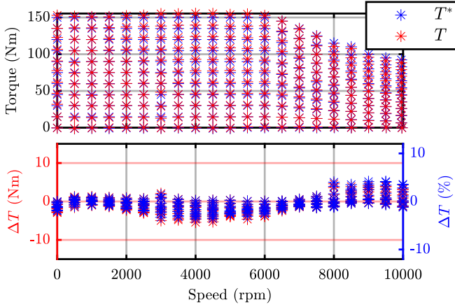
Fig. 22: Steady-state torque accuracy: experimental results.
