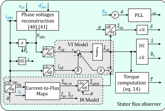
Fig. 4: Schematic view of the adopted stator flux observer.
