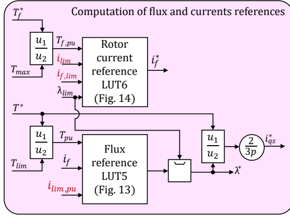
Fig. 12: Schematic view of the computation of flux and currents references.
