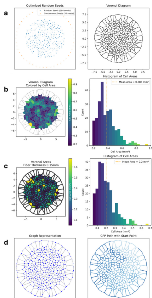
Fig. 4 (a) Visual representation of the generating seeds and the corresponding Voronoi pattern, (b and c) analysis of the pore area, related to input fiber thicknesses of 0 and 0.15 mm, respectively, (d) graph visualization and relative path to travel all the edges.
