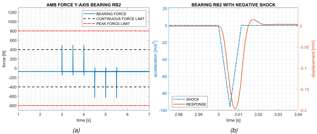
Figure 6: (a) Forces experienced by RB2 in y-axis due to shocks, constant radial compressor loads, and effect of static unbalance. (b) Displacement response of RB2 to a negative shock.
