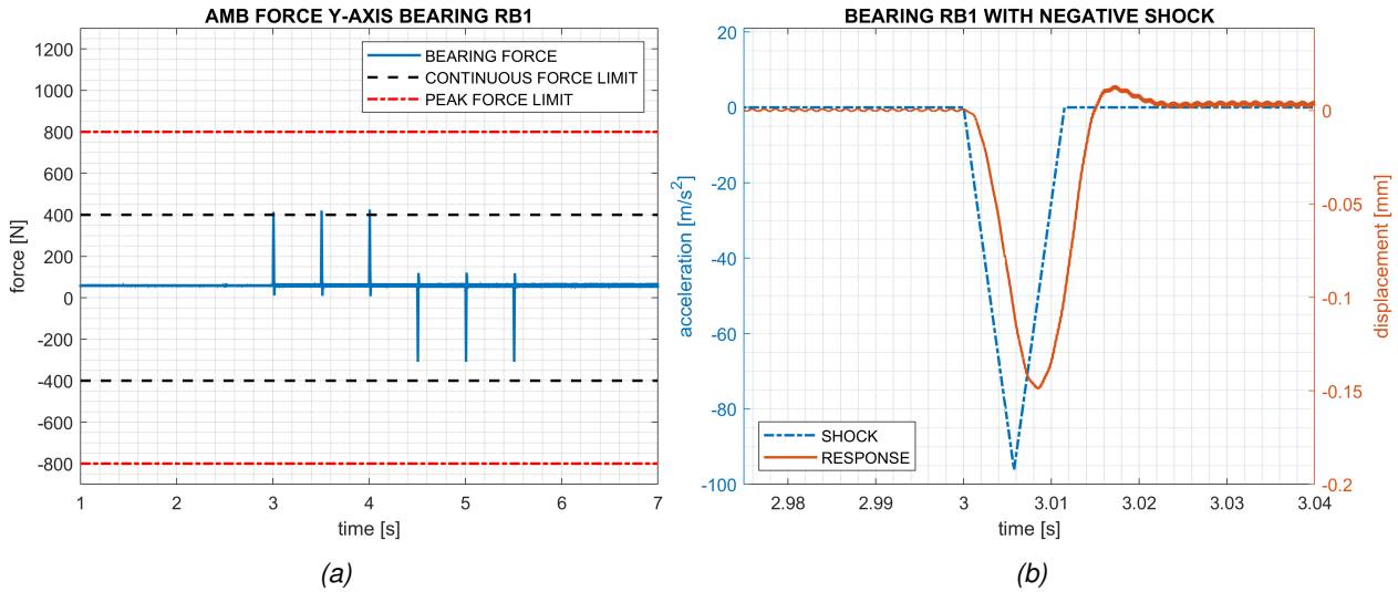
Figure 5: (a) Forces experienced by RB1 in y-axis due to shocks, constant radial compressor loads, and effect of static unbalance. (b) Displacement response of RB1 to a negative shock.
