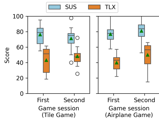
Figure 5: Comparison of SUS and TLX scores by session order for the Tile Game (left) and the Airplane Game (right).
