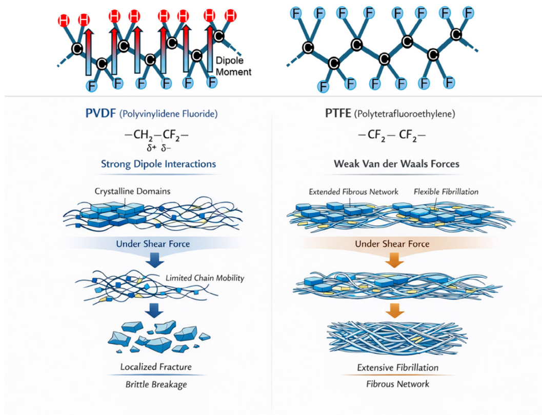
FIGURE 13 | Molecular structures and mechanical behaviors of PVDF and PTFE under shear force.
