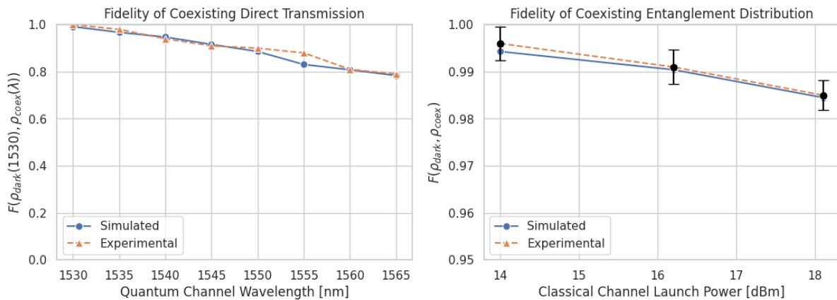
Fig. 1. Experimental and simulated quantum state fidelities of coexisting (a) direct transmission versus quantum channel wavelength, and (b) entanglement distribution versus launch power.
