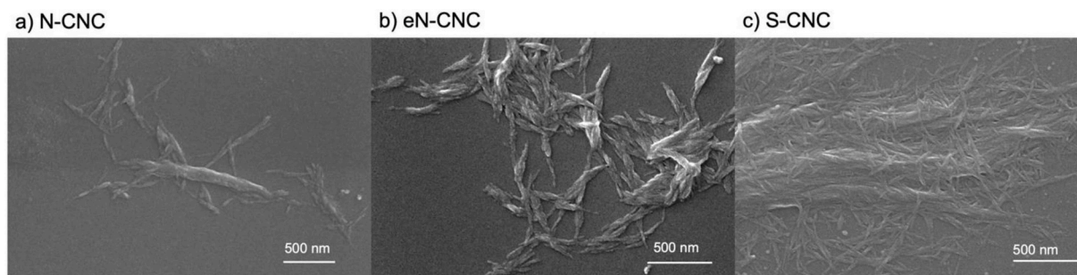
Fig. 4. FESEM micrographs of: a) N-CNC; b) eN-CNC; c) S-CNC, acquired on samples deposited on glass from 1 mg L -1 DMSO suspensions.
