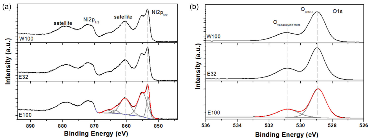
FIGURE 6 | XPS (a) Ni 2p and (b) O 1s regions for all three samples. In the E100 graphs, a deconvolution procedure, following Biesinger et al. [50], has been applied and reported.
