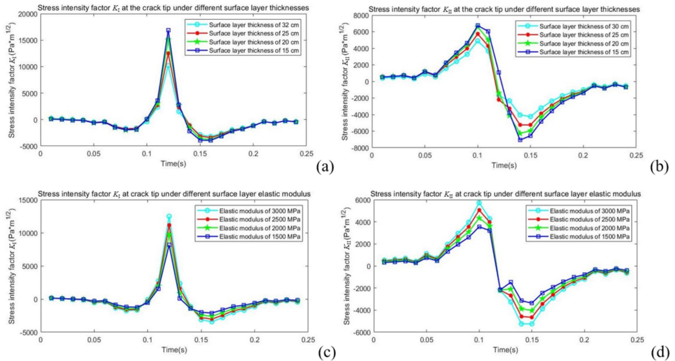
Fig. 6 Curves of stress intensity factors K_I and K_{II} at the crack tip with different surface layer thicknesses and elastic moduli: (a, b) K_I and K_{II} for different surface layer thicknesses, (c, d) K_I and K_{II} for different surface layer elastic moduli
