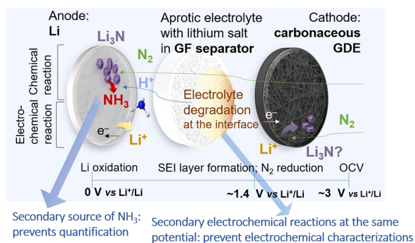
Figure 6. Schematic representation of the chemical and electrochemical reactions of a \text{Li}-\text{N}_2 cell (with relative potentials vs \text{Li}^+/\text{Li} ), pointing out the main limitations of this setup.
