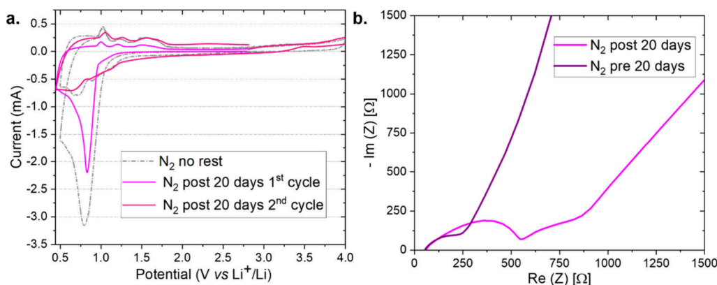
Figure 3. (a) CV traces at 0.1 mV s -1 of sealed coin cells assembled with a lithium anode, 1.55 mm-thick GF separator soaked in 1 M LiCF 3 SO 3 in TEGDME, and GDL. The gray curve is obtained without any rest period, while the pink and red curves represent the first and second cycle, respectively, of a coin assembled under N 2 and tested with CV after 20 days of rest. (b) EIS measurement of the same cell assembled under N 2 just after cell assembly (purple line) and after 20 days of rest (pink line); in the latter case, the EIS experiment was performed just before the CV presented in (a).
