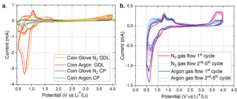
Figure 2. (a) CV traces at 0.1 mV s -1 for coin cells with holed caps, tested in different glovebox environments, assembled with a lithium anode, 1.55 mm-thick GF separator soaked in 1 M LiCF 3 SO 3 in TEGDME, and GDL (red and orange) or CP (pink and green) as the cathode. The cells were tested under argon (red and green) or in a N 2 -filled glovebox (orange and pink). (b) CV traces at 0.1 mV s -1 for EL-Cells assembled with a lithium anode, 1.55 mm-thick GF separator soaked in 1 M LiCF 3 SO 3 in TEGDME, and CP, tested after 30 min of rest (aimed to reach electrolyte saturation), maintaining a constant gas flow of filtered argon (green) or N 2 (purple) at 4 mL min -1 .
