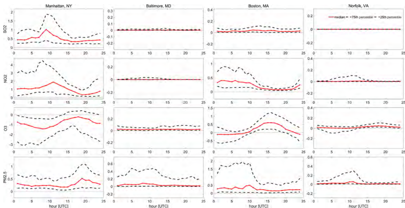
Figure 11. Diurnal cycle of the ship emission impacts on pollutants for (a) SO 2 (ppb), (b) NO 2 (ppb), (c) O 3 (ppb), and (d) PM 2.5 ( \mu\text{g m}^{-3} ). The first through fourth columns represent respective changes in Manhattan, NY; Baltimore, MD; Boston, MA; and Norfolk, VA.
