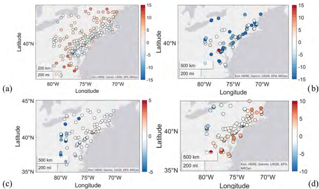
Figure 4. CAMx model performance against the AirNow observations: the MBE calculated at each station for (a) O 3 (ppb), (b) NO 2 (ppb), (c) SO 2 (ppb), and (d) PM 2.5 (μg m -3 ). Blue shades show a systematic underestimation, whereas red shades illustrate a systematic overestimation by the model.
