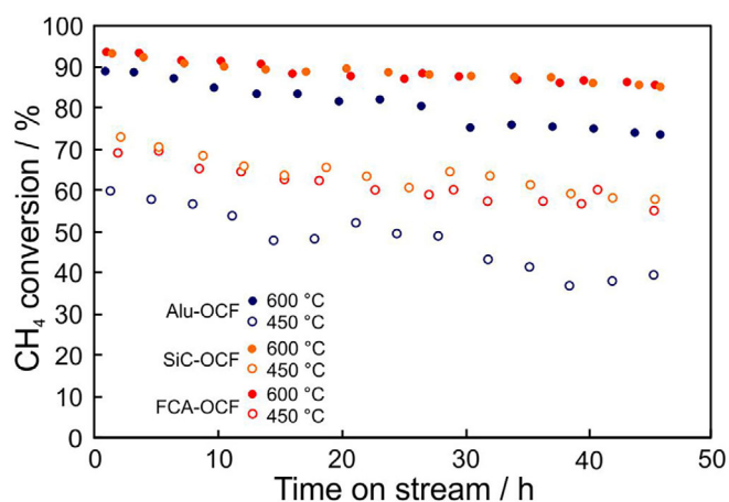
FIGURE 7 | Hydrothermal aging during 45 h with 10 vol.% H 2 O of different PdO/Co 3 O 4 coated OCFs.
