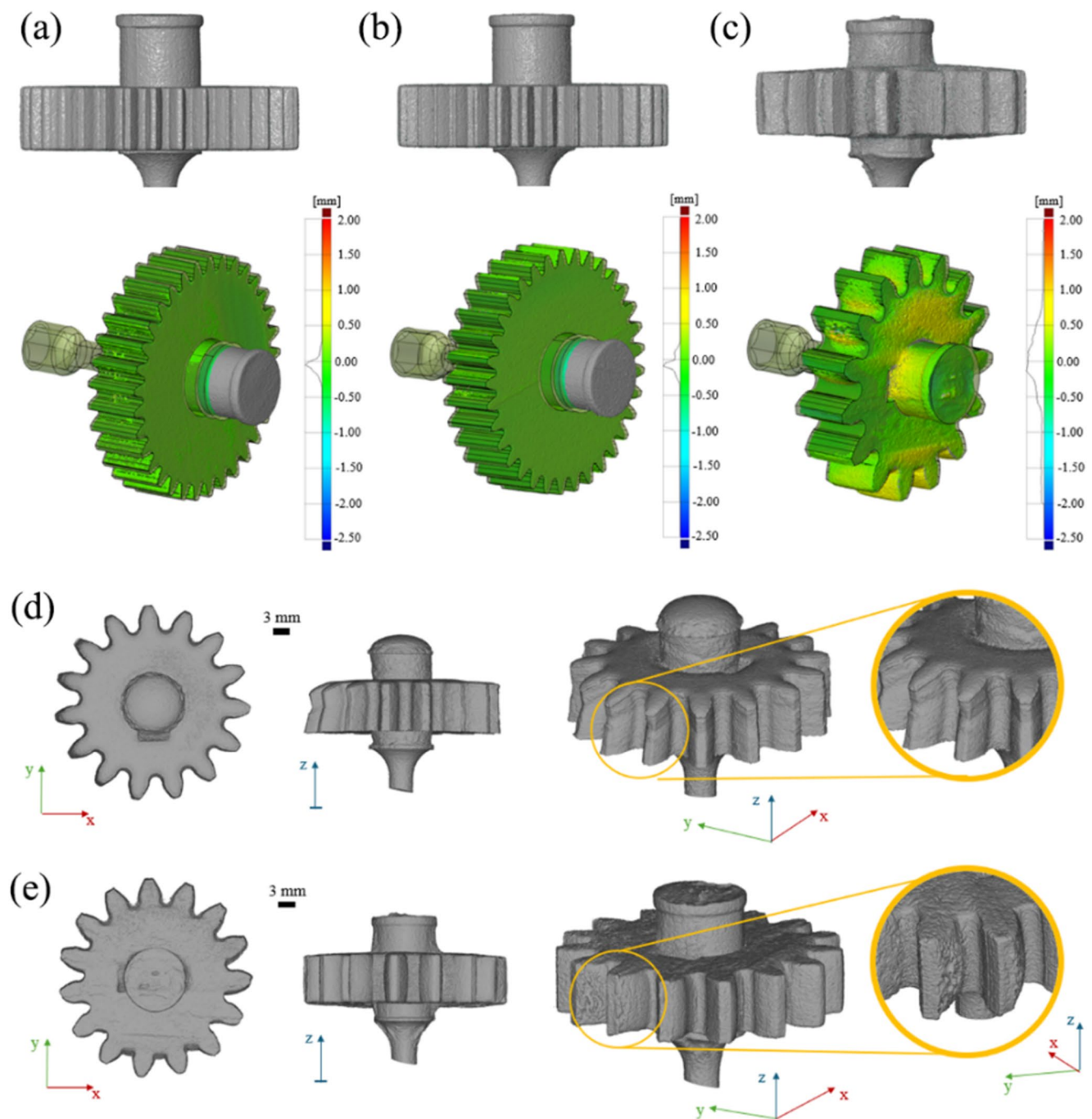
Fig. 7 Ct scan images. (a–c) Comparison with the CAD model: (a) Sample H1_8 , virgin powder; (b) sample V1_8 , virgin powder; (c) sample V2_{10_g} , refreshed powder, approximately 86 h. (d) Sample H2_{10_g} , (e) sample V2_{10_g}
