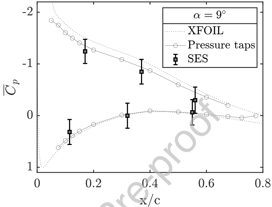
Figure 3: Comparison between the pressure coefficient measured with pressure taps (circles) and with the SES (squares): nacelle-only case as well as estimated with XFOIL (dotted line).
