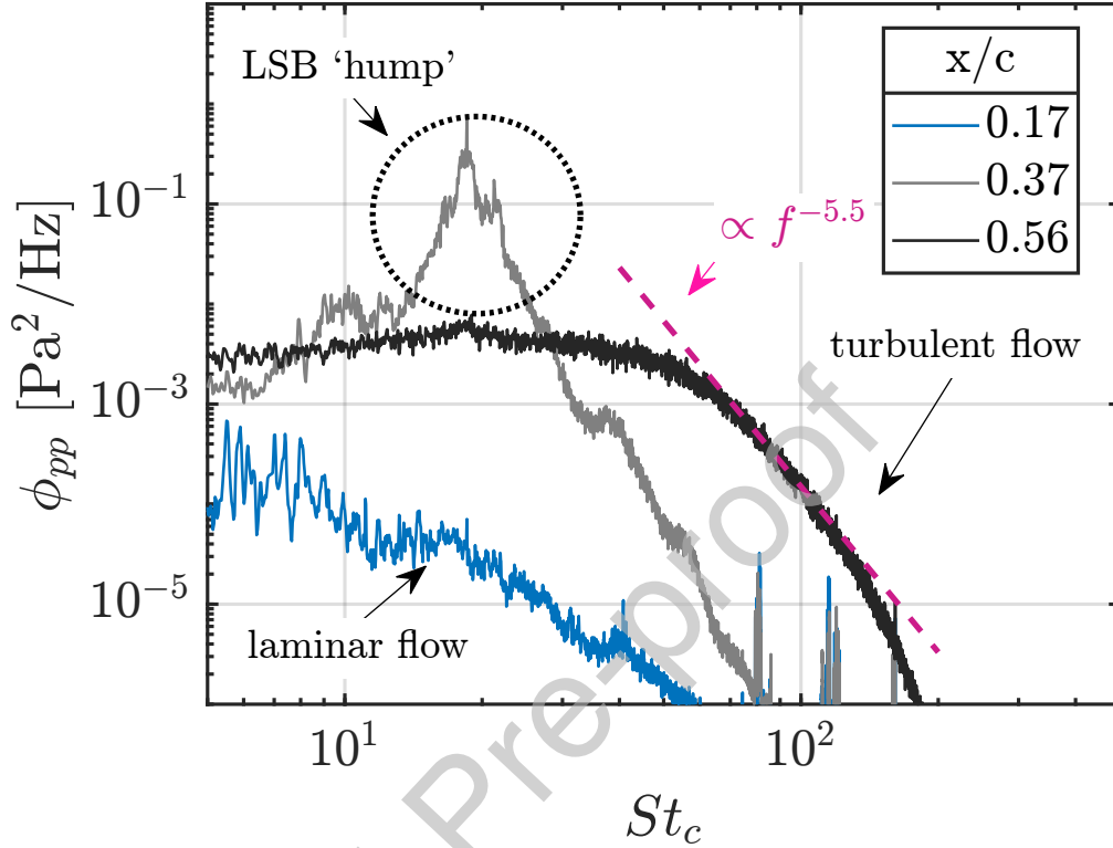
Figure 7: Wall pressure PSD measured at y/c = 0.4 for \alpha = 6^\circ at 20 m/s, nacelle-only case.
