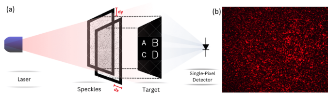
Fig. 1. (a) Conceptual illustration of the imaging process. (b) Example of speckle pattern on glass plate, acquired by a Thorlabs DCC1645C CMOS camera with resolution of 1280 \times 1024 pixels and 3.6 \mu\text{m} \times 3.6 \mu\text{m} pixel size.
