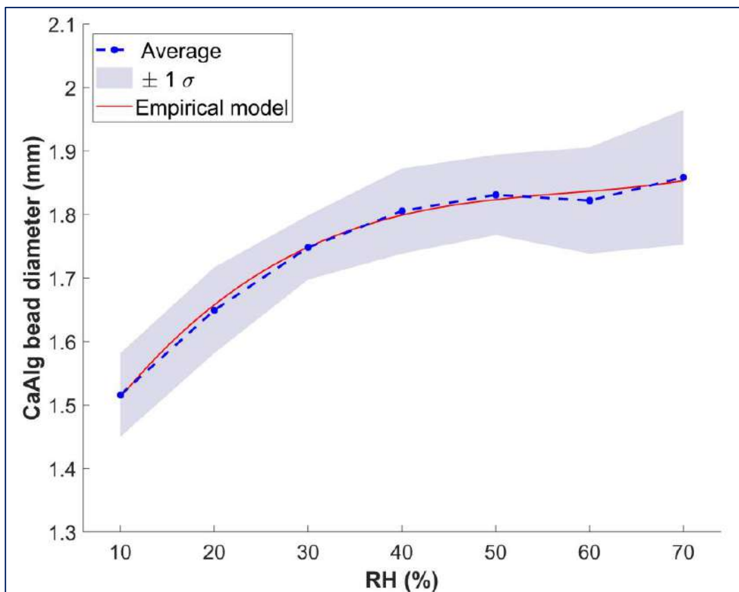
Figure s21: Relationship between equilibrium RH and CaAlg beads diameter, at T=30^{\circ}\text{C} . The blue dotted line connects the experimental measurements, each taken as average over 10 beads (per each bead, three diameters were averaged, for a total of 30 measurements per each RH). The blue background area encloses \pm one standard deviation calculated on the 10 beads considered at each RH. The red curve corresponds to the best-fitting cubic curve: D(\text{RH})=2.41 \cdot (\text{RH}/100)^3 - 4.19 \cdot (\text{RH}/100)^2 + 2.55 \cdot (\text{RH}/100) + 1.30 .
