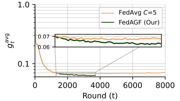
Fig. 2. Gradient feedback signal ( g_t^{\text{avg}} ) during training on CIFAR-100 with L \leq 5 [12].
