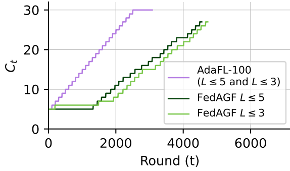
Fig. 3. Concurrency evolution ( C_t ) during training on CIFAR-100 with AdaFL and FedAGF.
