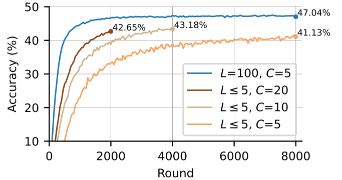
Fig. 1. Accuracy during training on CIFAR-100 with different label distributions ( L ) and concurrency levels ( C ) [12].
