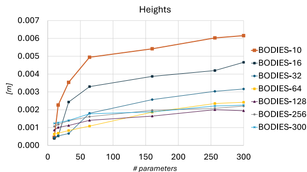
Fig. 15 Plots showing the progression of the error in the considered body measurement (the height) computed for the female subjects as a function of the number of parameters used to describe them in the test set, for all the considered configurations. The Integral Value (IV) for a given configuration is the area under the corresponding plot.
