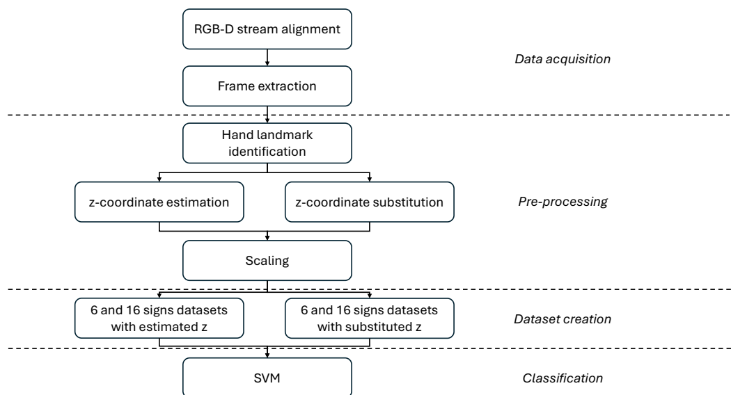
Figure 1. Workflow of gesture recognition.
