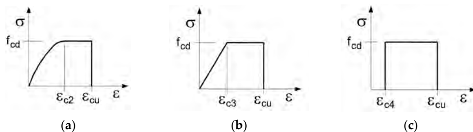
Figure 1. NTC 2018 [18] concrete constitutive laws: rectangular–parabolic (a), triangular–parabolic (b) and (c) rectangular “stress-block”.
