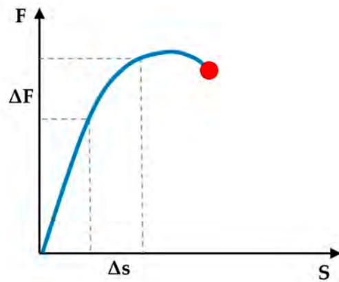
Figure 15. Force-controlled analysis [17].
