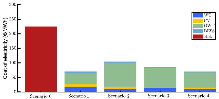
Fig. 21. Cost of energy resulting from the chosen scenarios and comparison with the 2022 price.
