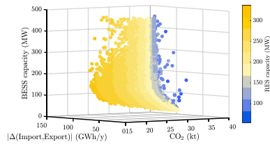
(c) Case 5 optimisation outcomes: 50% EV scenario: different installed RES capacities and the resulting relative CO 2 emissions, |Δ(Import, Export)| and installed BESS capacity effect on the system.
