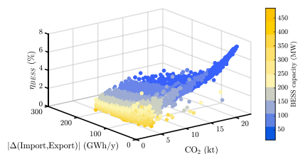
(a) Case 6 optimisation outcomes: 100% EV scenario: different installed BESS capacities and the resulting relative efficiency terms, CO 2 emissions and |Δ(Import, Export)|.
