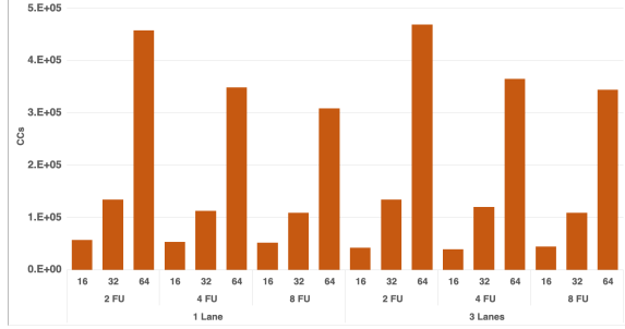
Fig. 4. CCs for different VPU configurations and data sizes
