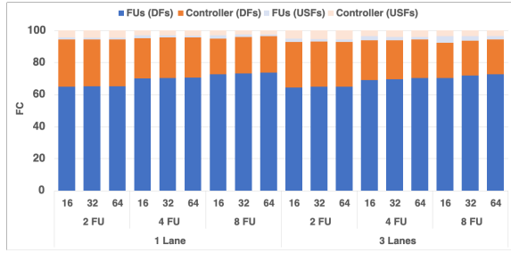
Fig. 3. Gate-level FC for different VPU configurations and data sizes
