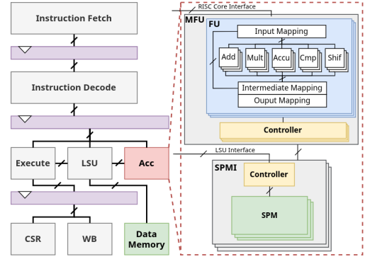
Fig. 1. A general scheme of the Klessydra-T block organization.
