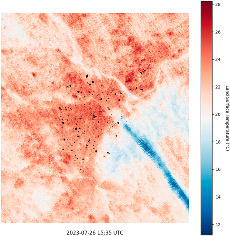
Figure 1. Example of processed ECOSTRESS satellite map of land surface temperature for Turin on 26 July 2023. Black polygons highlight the representative urban blocks selected through the morphology analysis.
