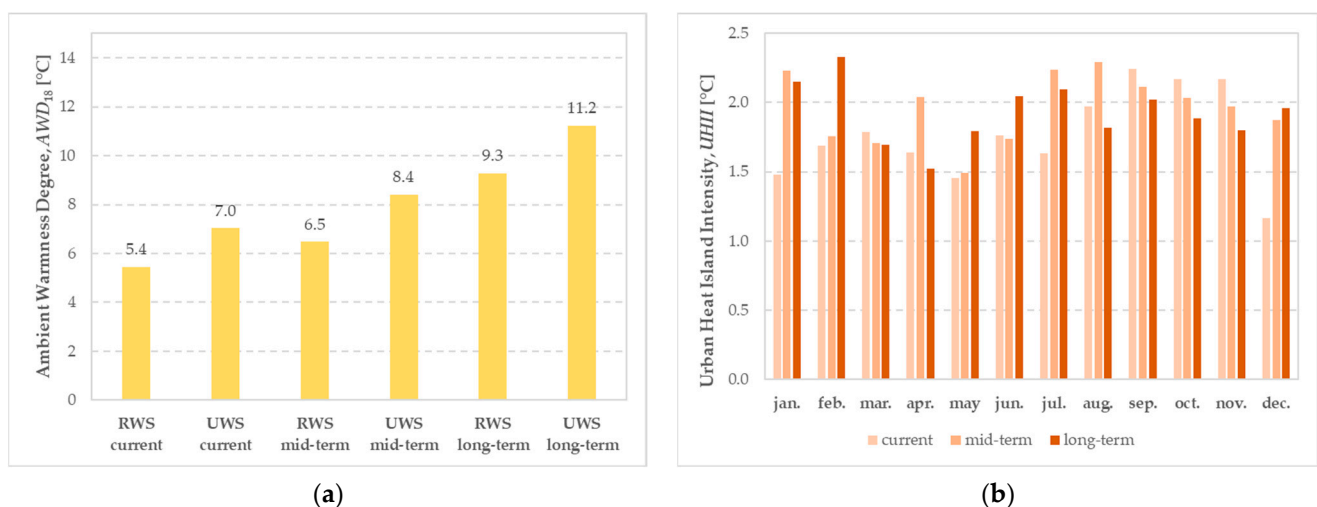
Figure 6. Ambient warmth degree (a) and urban heat island intensity (b) based on RWS and UWS data for the current, mid-, and long-term periods in urban block A.
