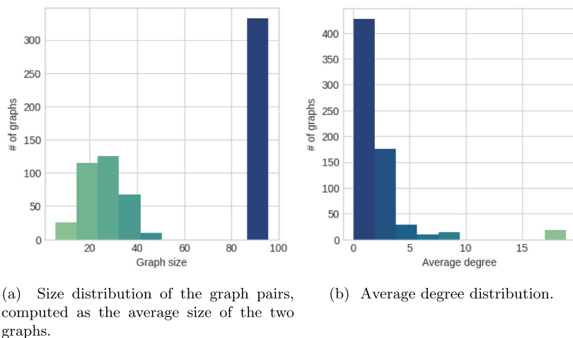
Fig. 2 Graph size distribution of the SMALL dataset
