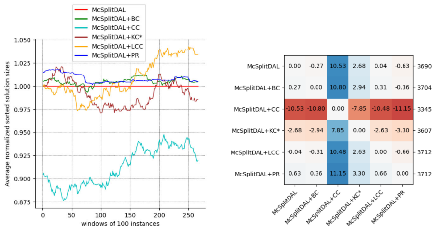
Fig. 5 Performance of McSplitDAL+X over the LARGE dataset
