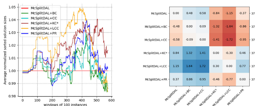
(a) Gain plot with a window width of 100 consecutive tests of the sizes of the solutions obtained by the McSplitDAL+X algorithms. All values are normalized with respect to the results obtained by McSplitDAL.
