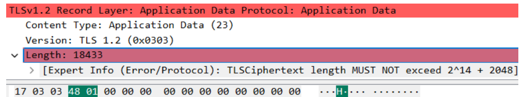
Figure 8. Wireshark dump showing the traffic generated in the test for a TLS Record whose size exceeds the limited allowed by the RFC ( 2^{14} + 2048 bytes).
