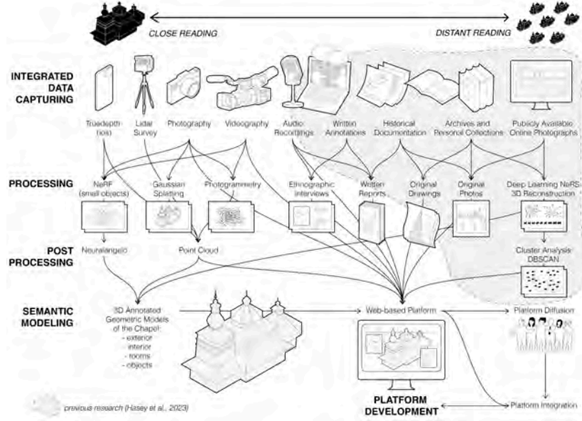
Fig. 2. Methods and pipeline for the capture, processing, and modeling through a variety of systems leading to the prototype.
