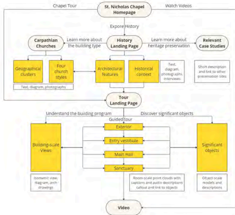
Fig. 8. Information architecture diagram of the interactive, web-based document (left). Linear presentation if scrolling through the webpage (right).
