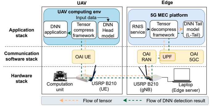
Fig. 2: Schematic representation of our testbed.
