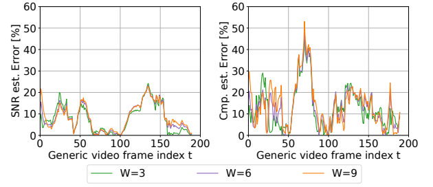
Fig. 7: Reconstructed tensor SNR (left) and tensor compression ratio (right): measurement and estimation.
