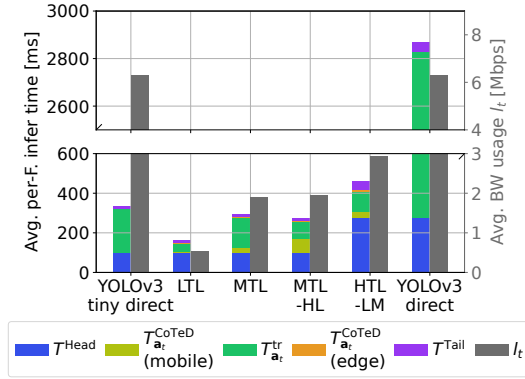
Fig. 15: Breakdown of average per-frame inference latency and average wireless bandwidth usage for CoTeD Manager orchestration and direct DNN splitting in target scenarios.
