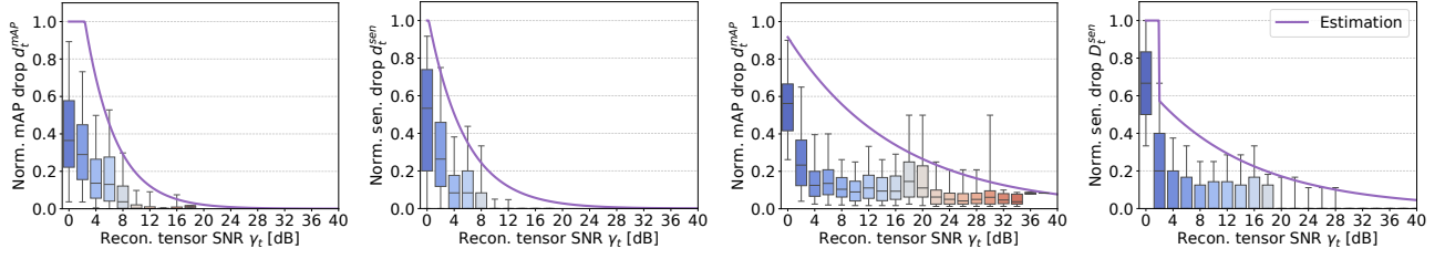
Fig. 6: Normalized DNN object detection mAP/sensitivity drop vs. SNR of the reconstructed tensor \hat{\mathbf{P}}_t for the BEV (left: mAP drop; middle-left: sensitivity drop) and, St. Marc (middle-right: mAP drop; right: sensitivity drop) datasets.
