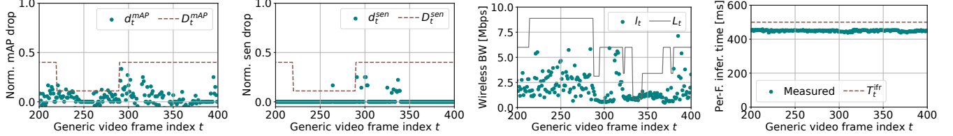
Fig. 14: HTL-LM scenario: CoTeD Manager orchestration performance: (left) Normalized DNN mAP drop, (middle-left) Normalized DNN sensitivity drop, (middle-right) Used wireless bandwidth, and (right) Per-frame inference time.
